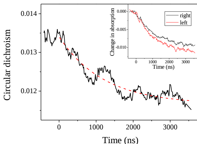
Figure 3. Circular dichroism in absolute value measured at 220 nm as a function of time. The inset shows the corresponding changes in absorption for the left and right circular polarization.
