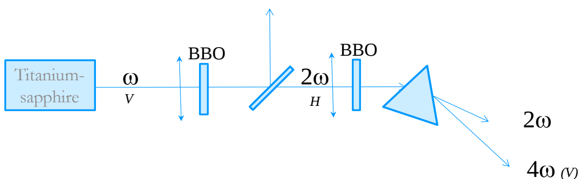
Figure 5. Schematic of the fourth harmonic generation of the 82 MHz Titanium-Sapphire laser. The letters V or H refer to the beam polarizations.
