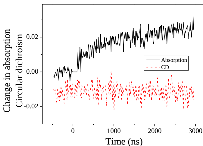
Figure 4. Change in absorption and circular dichroism measured at 204 nm as a function of time.
