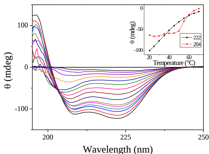
Figure 1. Circular Dichroism (CD) spectra of Poly(glutamic acid) (PGA) for 15 temperatures ranging from 7.7 to 70 °C. For this measurement, the PGA concentration was reduced to 7.5 mg/mL and the cell thickness was 100 \mu m. The inset shows the ellipticity measured at 204 and 222 nm as a function of the temperature.
