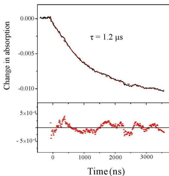
Figure 2. Change in absorption at 220 nm as a function of time. The dashed line is a monoexponential fit whose residual is displayed in the lower panel.
