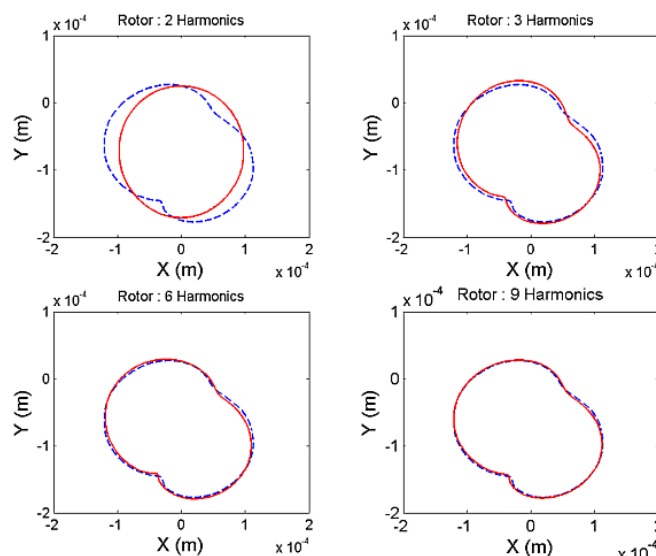
Figure 10. HBM AFT (—) and direct integration (---).
