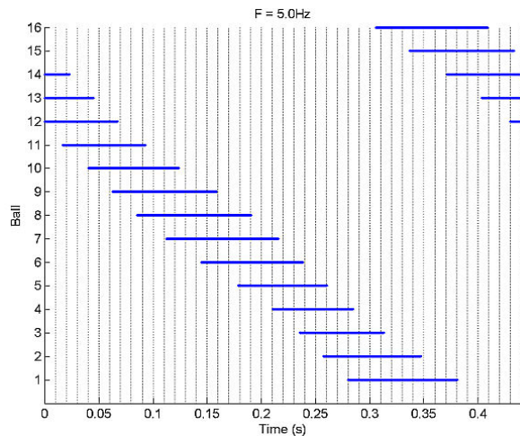
Figure 11. Contact time for each ball (F=5.0 Hz).
