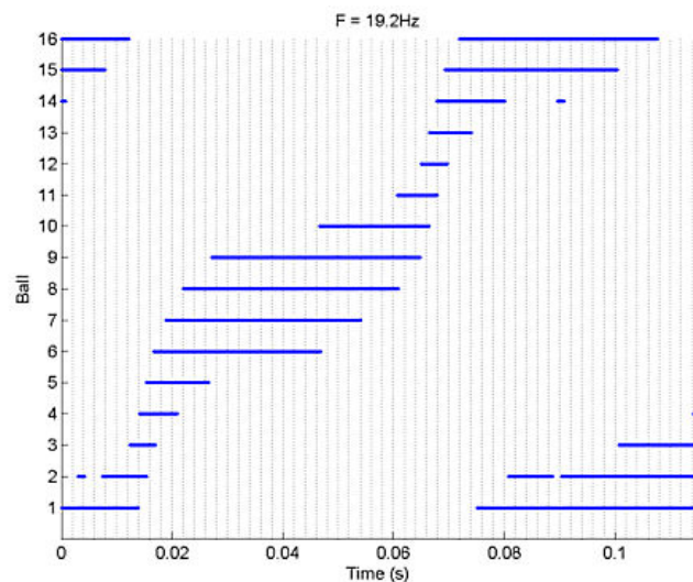
Figure 14. Contact time for each ball (F=19.2 Hz).
