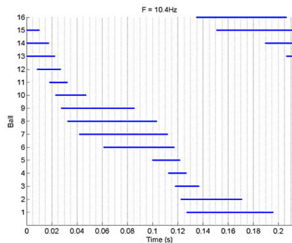
Figure 12. Contact time for each ball (F=10.4 Hz).
