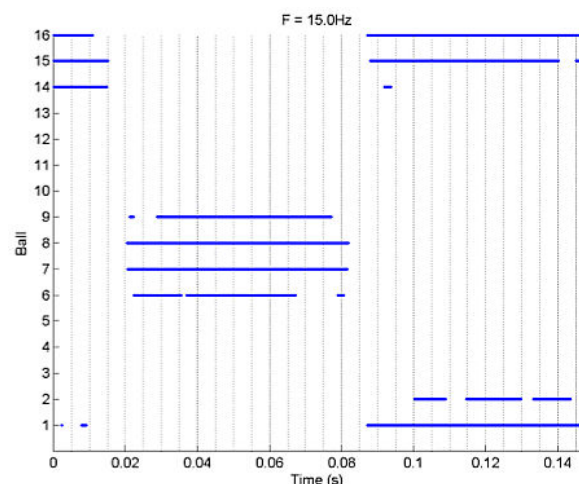
Figure 13. Contact time for each ball (F=15.0 Hz).
