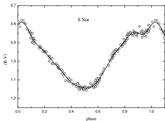
Figure 3. As in Fig. 2 but for S Nor.
