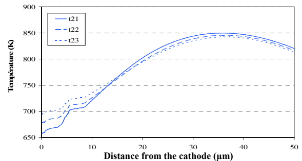
Figure 19 - 1D temperature evolution just after turn-off along a-a' cut line indicating an increase of the cathode temperature
