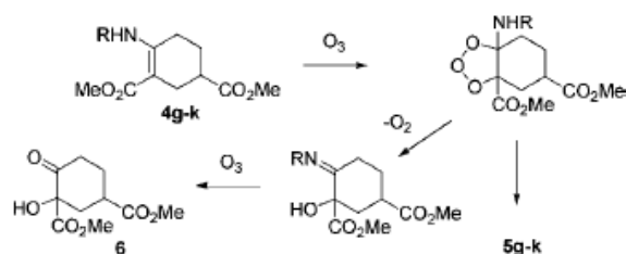
Scheme 3. Oxidation of Enamines 4g–k
