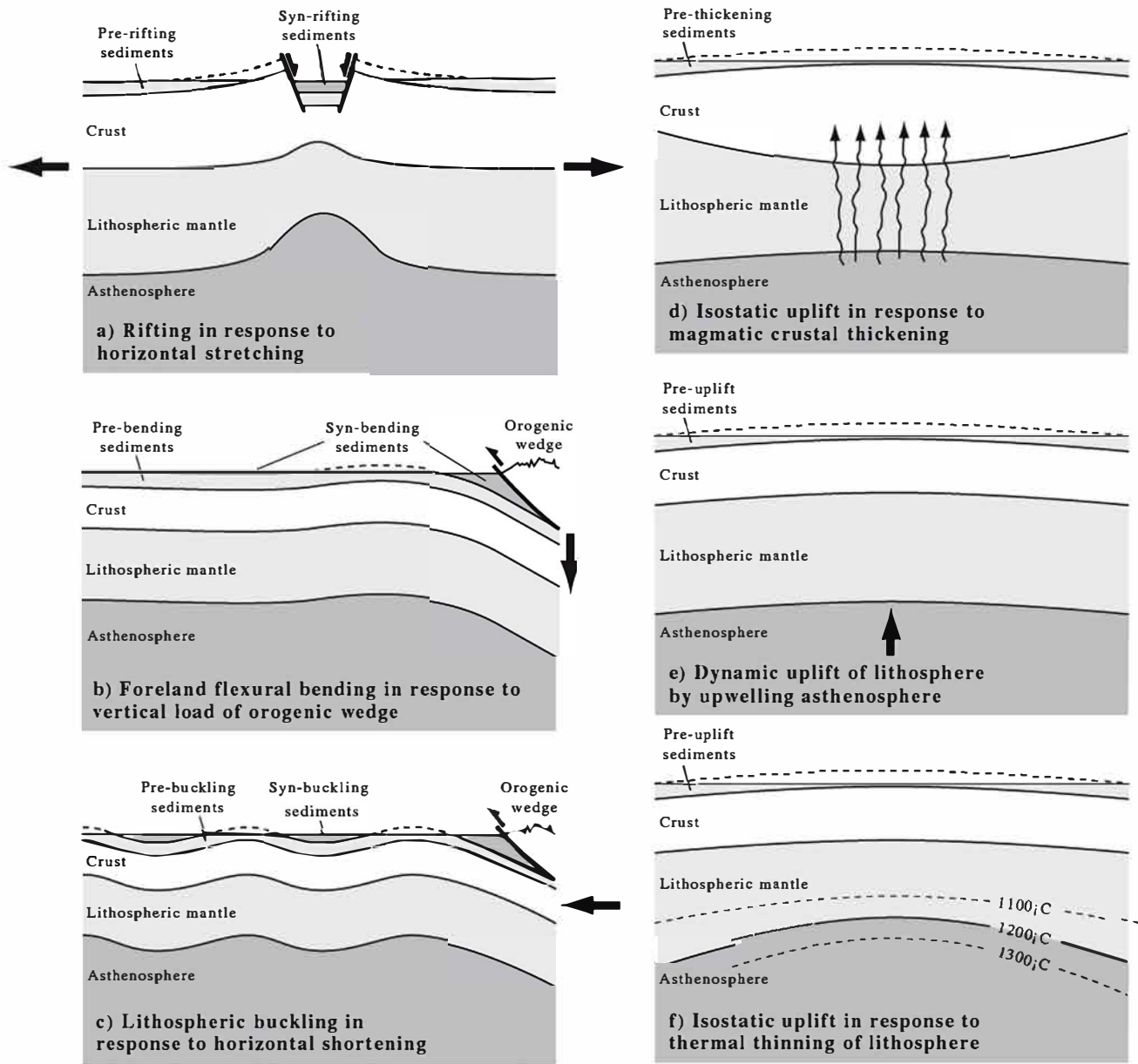
Fig. 4 Sketches (not to scale) of theoretical geometrical signatures of a) rifting, b) foreland flexural bending, c) lithospheric buckling, d) magmatic crustal thickening, e) dynamic uplift of lithosphere by up
