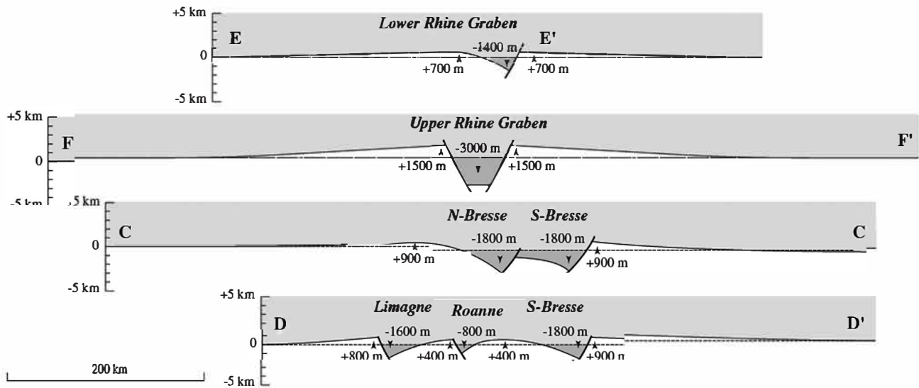
Fig. 8 Map and cross sections of rift signature on top basement in the NW Alpine foreland. Contours indicate amounts of vertical motions of the basement caused by rifting. Positive values indicate uplift (graben shoulders) and negative values indicate subsidence
