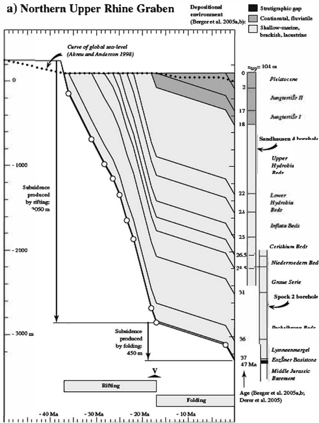
◀ Fig. 12 Accumulation curves computed for a) the northern part and b) the southern part of the Upper Rhine Graben. Timing of volcanic activity (K Kaiserstuhl, V Vogelsberg) after Sissingh (2003) and Berger et al. (2005a, b)
