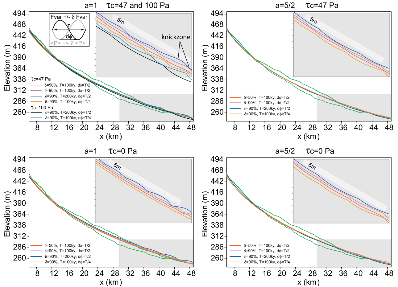
Figure 5. Effect of variable climate. The Ill and Lague profiles are in green. The model profiles are computed by imposing sinusoidal variations to the mean precipitation rate \langle P \rangle and to the variability factor F_{var} . The reference mean values are \langle P \rangle = 500 \text{ mm yr}^{-1} and F_{var} = 10 and the constant uplift rate relative to the pinned bottom condition is U = 0.1 \text{ mm yr}^{-1} . The fitting results are given in Table 3. Inset gray diagrams show an enlargement of the last 20 km of the profiles. The profiles have been slightly shifted vertically for ease of viewing. A 5-m ruler is displayed to measure the amplitude of elevation changes because of climate oscillations. These figures show that elevation changes along a single profile are smaller than 5 m whatever the tested scenario and erosion parameters. This suggests that climate variations cannot explain the main knickzone along the Ill River.
