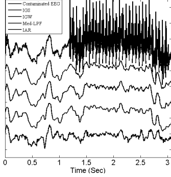
Figure 4: Comparison of methods in reducing MR artifact from EEG signal. From up to bottom, contaminated EEG signal with MR artifact, the processed signal by IGS, IGW, Med-LPF, and IAR.
