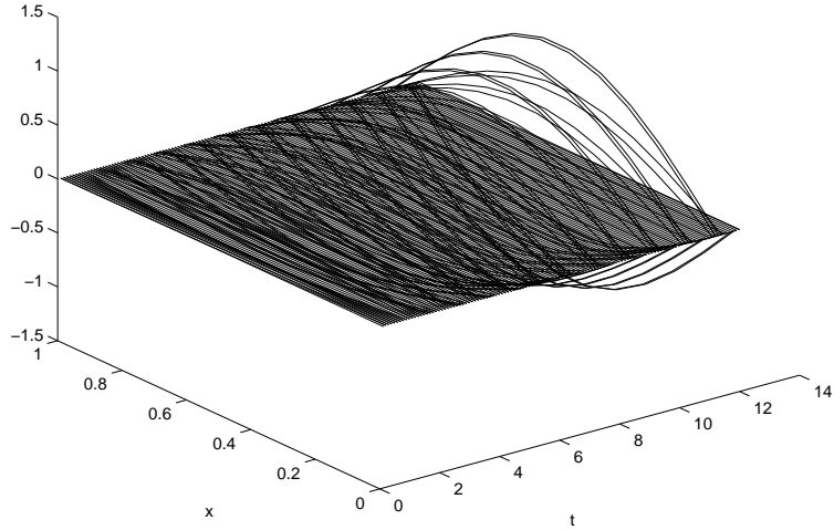
Figure 2: Numerical solution
