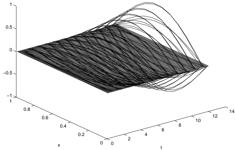
Figure 3: Exact solution
