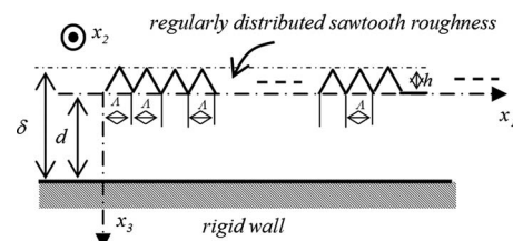
FIG. 3. Fluid plate between two rigid walls: the smooth plane wall and the wall having regularly distributed corrugations (sawtooth profile).
