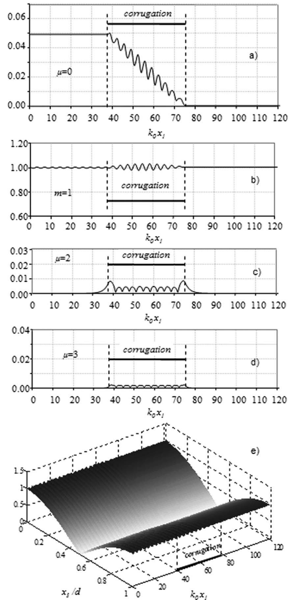
FIG. 5. Modulus of the normalized amplitude of the pressure variation (third order) for the sawtooth profile (see Fig. 3). (a) \hat{A}_{\mu=0}^{[3]}(x_1)/A_m^0 for mode \mu=0 , (b) \hat{A}_{m=1}^{[3]}(x_1)/A_m^0 for mode m=1 (the only mode generated by the source), (c) \hat{A}_{\mu=2}^{[3]}(x_1)/A_m^0 for the evanescent mode \mu=2 , (d) \hat{A}_{\mu=3}^{[3]}(x_1)/A_m^0 for the evanescent mode \mu=3 , and (e) the total pressure variation |\hat{P}^{[3]}(x_1)/A_m^0| , when fd/c_0=0.91 and d/\Lambda=5/3 . The coordinates of the ends of the corrugation are x_i and (x_i+\ell) with k_0x_i=37.7 ; the length \ell of the corrugation at x_3=0 being such that k_0\ell=37.7 , which corresponds to N=11 crenels (see Table I for dimensional quantities) and to \ell \approx 6\lambda for the fictitious glass fluid indicated in Table I. The heights of the teeth are such that h/d=0.005 ; the interface x_3=d is smooth (see Fig. 3).
