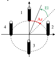
Figure 6: Array configuration.
