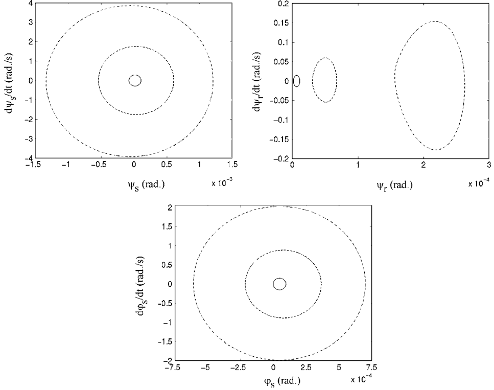
Fig. 22. Parametric studies for the \psi_s , \psi_r and \phi_s -limit cycles amplitudes ( \mu = 1.1\mu_0 ); — P_{\text{hydraulic}} = 10 bars, --- P_{\text{hydraulic}} = 15 bars, -.- P_{\text{hydraulic}} = 20 bars.
