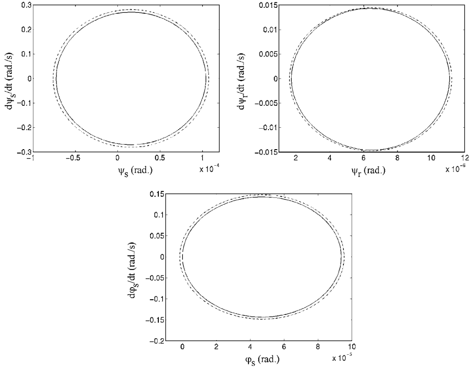
Fig. 18. \psi_s , \psi_r and \phi_s -limit cycles by using the centre manifold, the rational approximants and the alternating frequency/time method ( \mu = 1.1\mu_0 ); — original system, --- non-linear methods.
