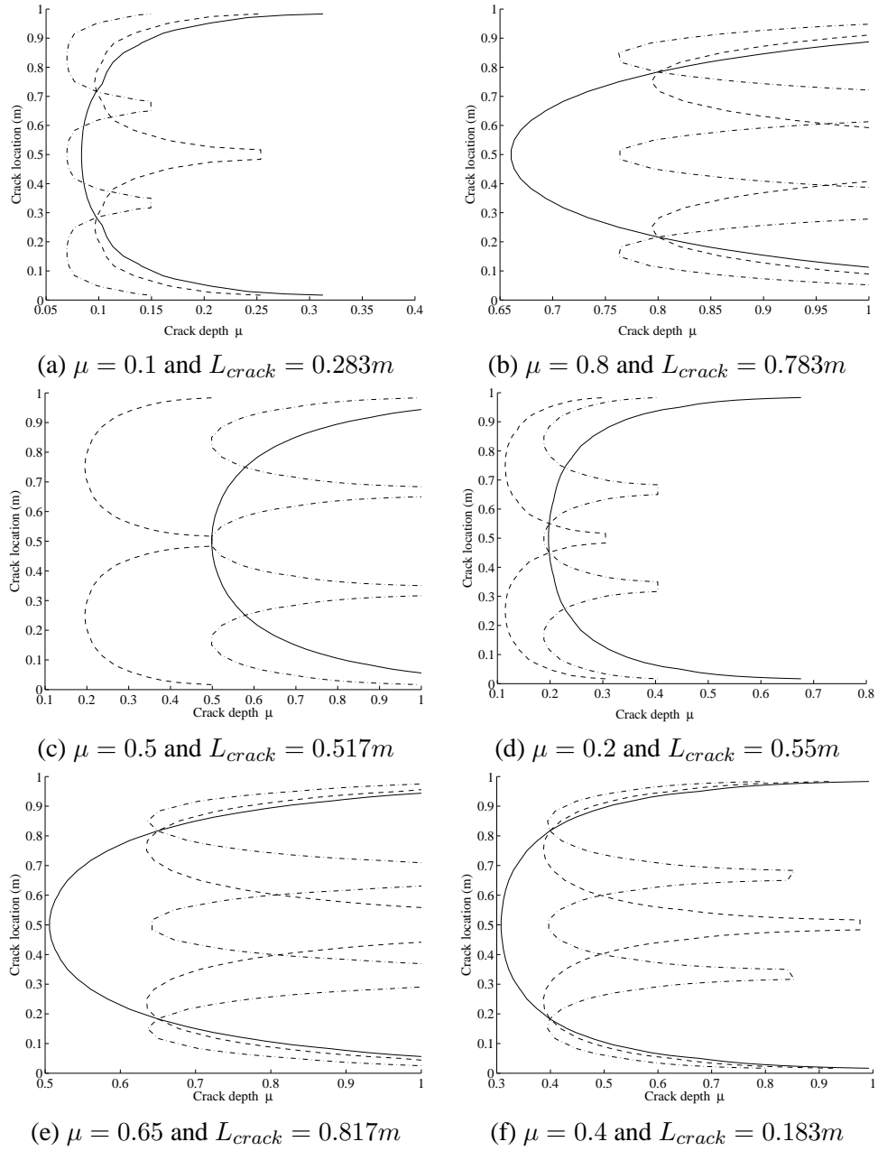
Figure 4: Identification results with the criterion \% \Delta_i^{cracked} by using the contour lines of the first three frequency ratios for a simply supported beam ( \text{— } \% \Delta_1^{cracked} , \text{-- -- } \% \Delta_2^{cracked} , \text{- . - } \% \Delta_3^{cracked} )
