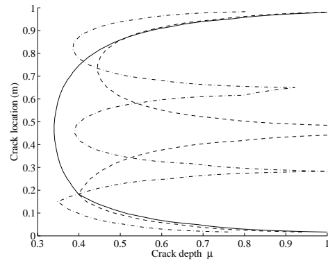
(f) \mu = 0.4 and L_{crack} = 0.183m
