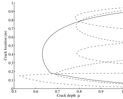
(b) \mu = 0.8 and L_{crack} = 0.783m
