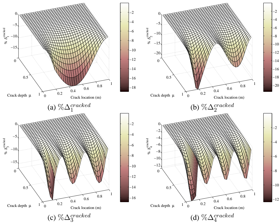
Figure 6: Evolution of \% \Delta_i^{cracked} of the beam with an added mass at L_{mass} = 0.167m as a function of the non-dimensional crack depth \mu and the crack location L_{crack} ( \text{---} \% \Delta_1^{cracked} , \text{-- --} \% \Delta_2^{cracked} , \text{- . -} \% \Delta_3^{cracked} )
