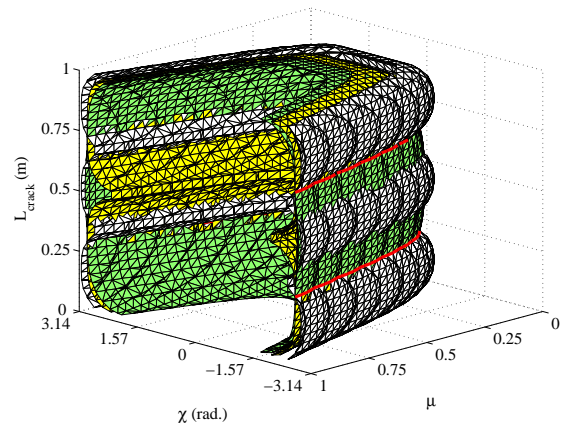
(b) \mu = 0.5, \chi = \frac{2\pi}{3}rad., L_{crack} = 0.28m
