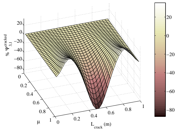
(a) \% \Psi_{3,1}^{cracked} for \chi = 0 \text{ rad} .
