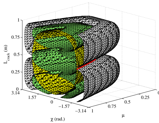
(c) \mu = 0.7, \chi = \frac{\pi}{2}rad., L_{crack} = 0.48m
