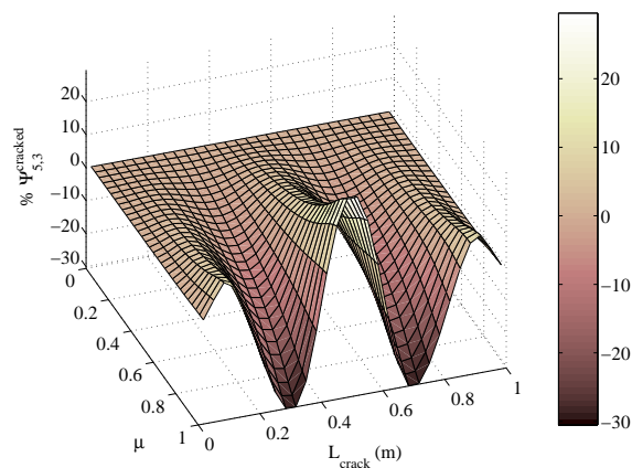
(e) \% \Psi_{5,3}^{cracked} for \chi = 0 \text{ rad} .
