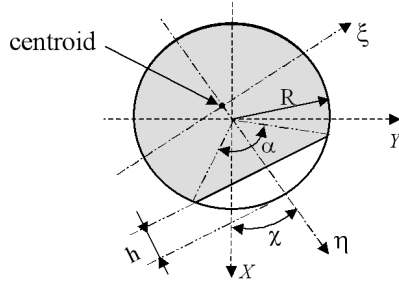
(a) Geometry of the cracked-beam section
