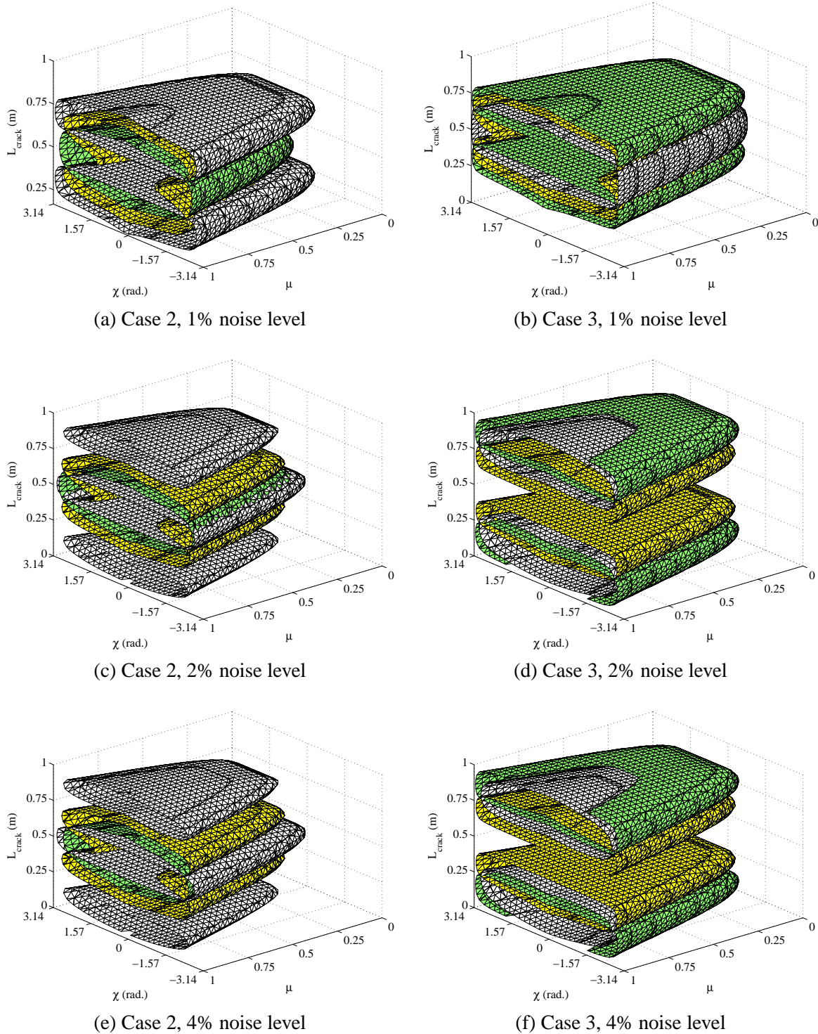
Figure 17 : Surfaces \% \Psi_{ij}^{cracked} with various noise levels for the case 2 ( \mu = 0.3, \chi = \frac{\pi}{3} rad. and L_{crack} = 0.62m ) and the case 3 ( \mu = 0.5, \chi = \frac{2\pi}{3} rad. and L_{crack} = 0.28m ) (green= \% \Psi_{31}^{cracked} , yellow= \% \Psi_{51}^{cracked} , white= \% \Psi_{53}^{cracked} )
