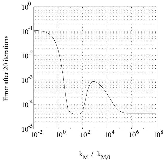
Figure 4: Traction-based micro-macro LATIN strategy: Error after 20 iterations.
