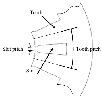
Figure 4. Geometry of the slot
