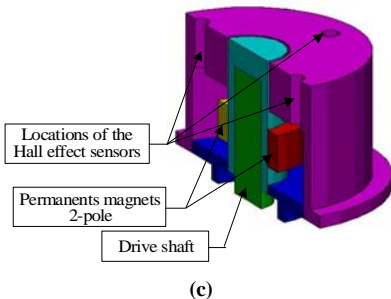
Figure 11. A PM position sensor. (a) Stator of PMPS, (b) "Image" of the turning parts motor, and (c) survey of PMPS
