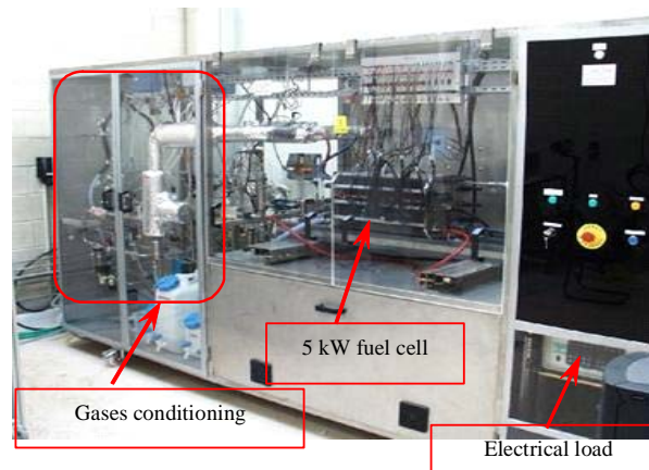
Figure 2. 5 kW FC test bench in the L2ES
