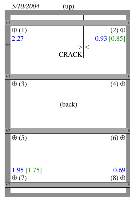
Fig. 2 Position and value of the reactions by of the crossbars on the panel
