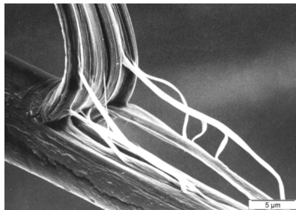
Figure 10 : Peeling of a fibrillable freeze-dried fibre
