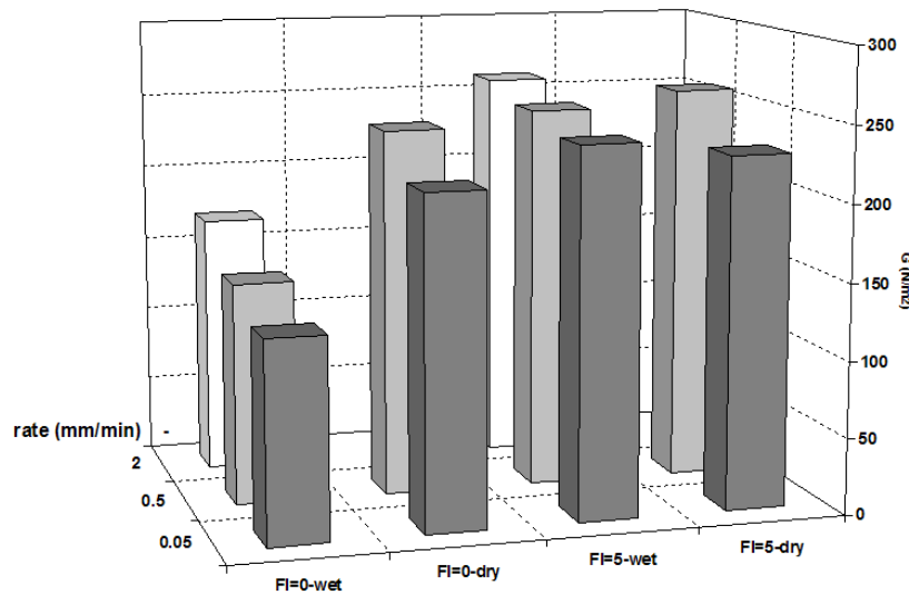
Figure 13: Energy release rate G for the different fibres as a function of peel rate
