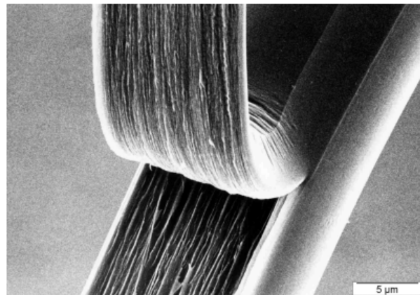
Figure 5 : Peeling of a non fibrillable freeze-dried fibre
