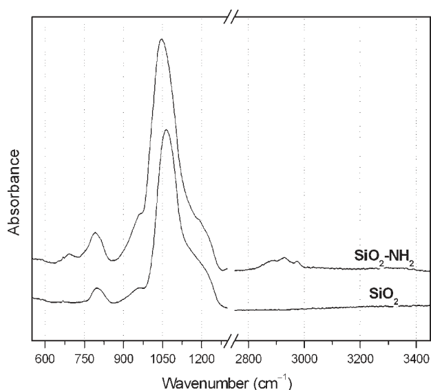
Fig. 3. FTIR spectrum for \text{SiO}_2 and \text{SiO}_2\text{-NH}_2 nanoparticles.
