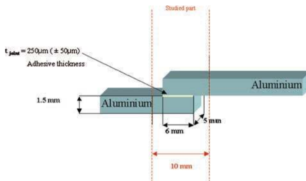
Fig. 2. Simple recovery joint aluminum assembly.
