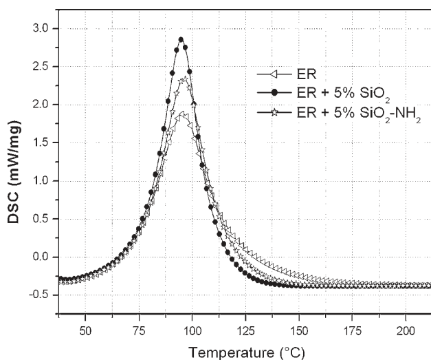
Fig. 7. Crosslinking rate curves of pure epoxy resin and its nanocomposites containing pure SiO 2 and SiO 2 -NH 2 .
