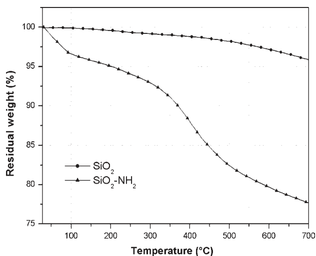
Fig. 5. Thermogravimetric curves for \text{SiO}_2 and \text{SiO}_2\text{-NH}_2 nanoparticles.
