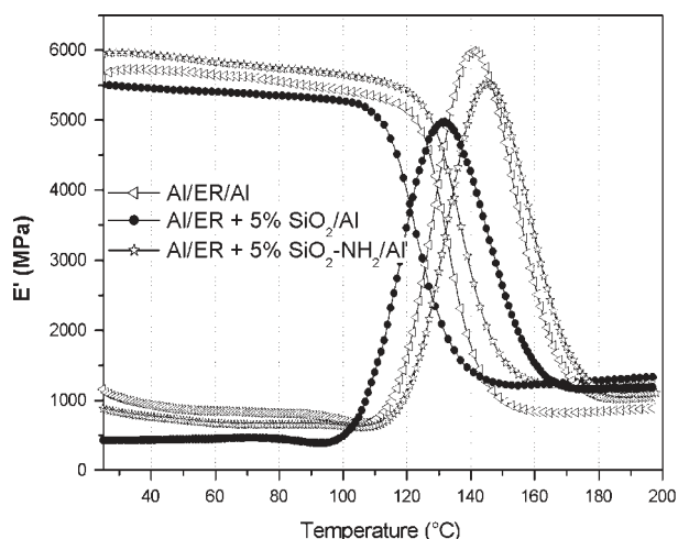
Fig. 9. DMA shear tests results of pure epoxy resin assembly and its nanocomposites containing pure \text{SiO}_2 and \text{SiO}_2\text{-NH}_2 .
