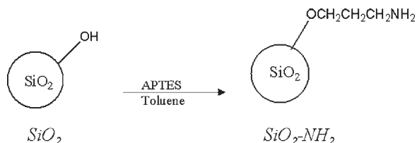
Fig. 1. Functionalization of nanosilica particles.
