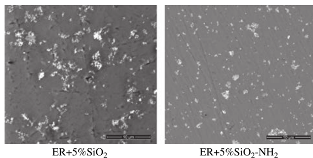
Fig. 6. SEM micrographs of epoxy/silica nanocomposites filled at 5 wt% of pure \text{SiO}_2 and \text{SiO}_2\text{-NH}_2 .
