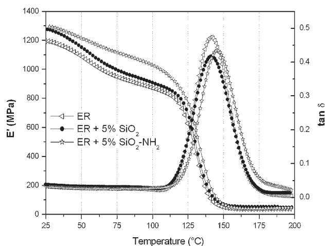
Fig. 8. DMA single cantilever results of pure epoxy resin and its nanocomposites containing pure SiO 2 and SiO 2 -NH 2 .
