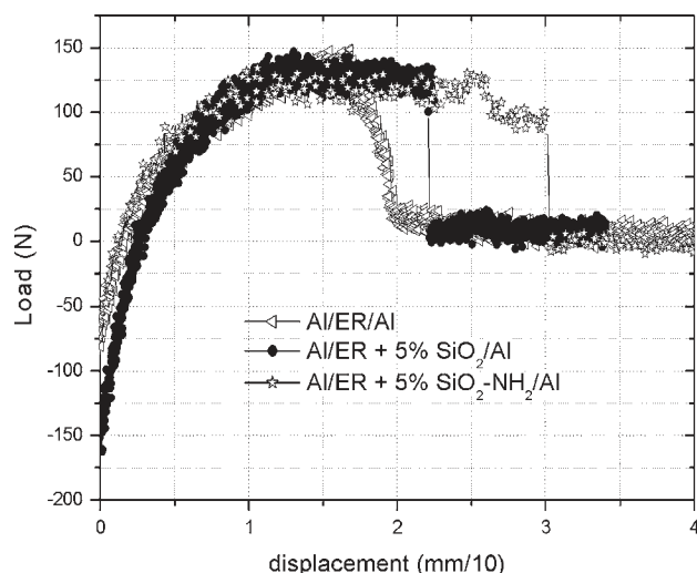
Fig. 10. Typical load–displacement curves for pure epoxy resin assembly and its nanocomposites containing pure \text{SiO}_2 and \text{SiO}_2\text{-NH}_2 .
