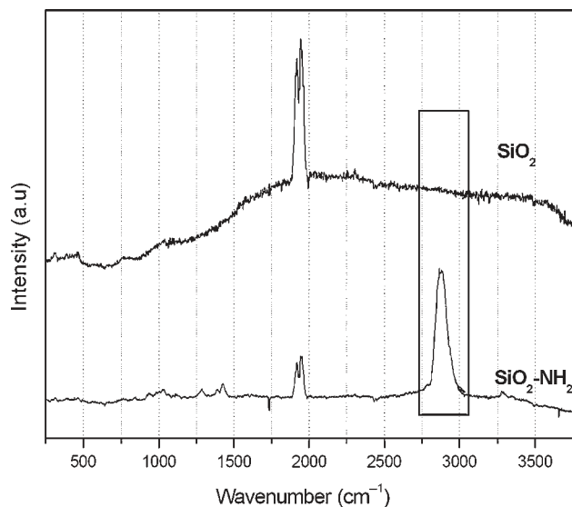
Fig. 4. Raman spectrum for \text{SiO}_2 and \text{SiO}_2\text{-NH}_2 nanoparticles.
