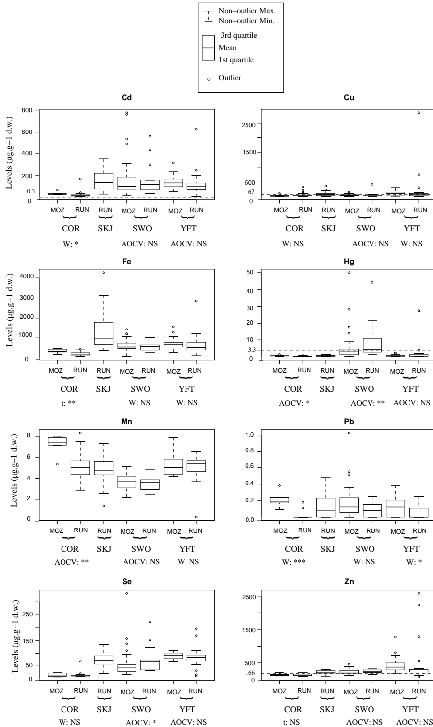
Fig. 3. Comparison of elemental levels ( \mu\text{g}\cdot\text{g}^{-1} d.w.) in liver of fish caught in the Mozambique Channel (MOZ) and Reunion Island waters (RUN). For each species, the significances of the level differences between both study sites are indicated below the boxplots. Horizontal dotted lines mark the European guidance levels for human consumption. COR: Common Dolphinfish; SKJ: Skipjack Tunas; SWO: Swordfish; YFT: Yellowfin Tunas; W: Wilcoxon test; t: t-test; AOCV: analysis of covariance; NS: Non significant.
