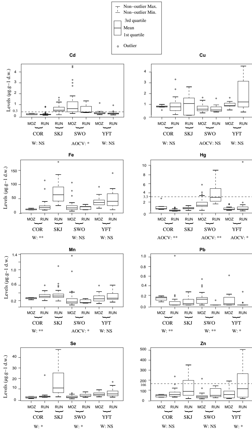
Fig. 2. Comparison of elemental levels ( \mu\text{g}\cdot\text{g}^{-1} d.w.) in muscle of fish caught in the Mozambique Channel (MOZ) and Reunion Island waters (RUN). For each species, the significances of the level differences between both study sites are indicated below the boxplots. Horizontal dotted lines mark the European guidance levels for human consumption. COR: Common Dolphinfish; SKJ: Skipjack Tunas; SWO: Swordfish; YFT: Yellowfin Tunas; W: Wilcoxon test; AOCV: analysis of covariance; NS: Non significant.
