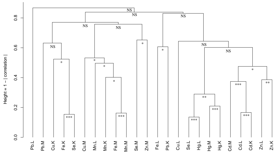
Fig. 5. Dendrogram illustrating linear correlations between trace elements in Swordfish. The minimum levels of significance of the linear correlation coefficients among groups of elemental levels are encoded in the dendrogram. NS: non significant. The letters “.L”, “.K”, “.M” and placed after the abbreviation of an element indicate the tissues (resp. liver, kidney and muscle) in which the element is considered.
