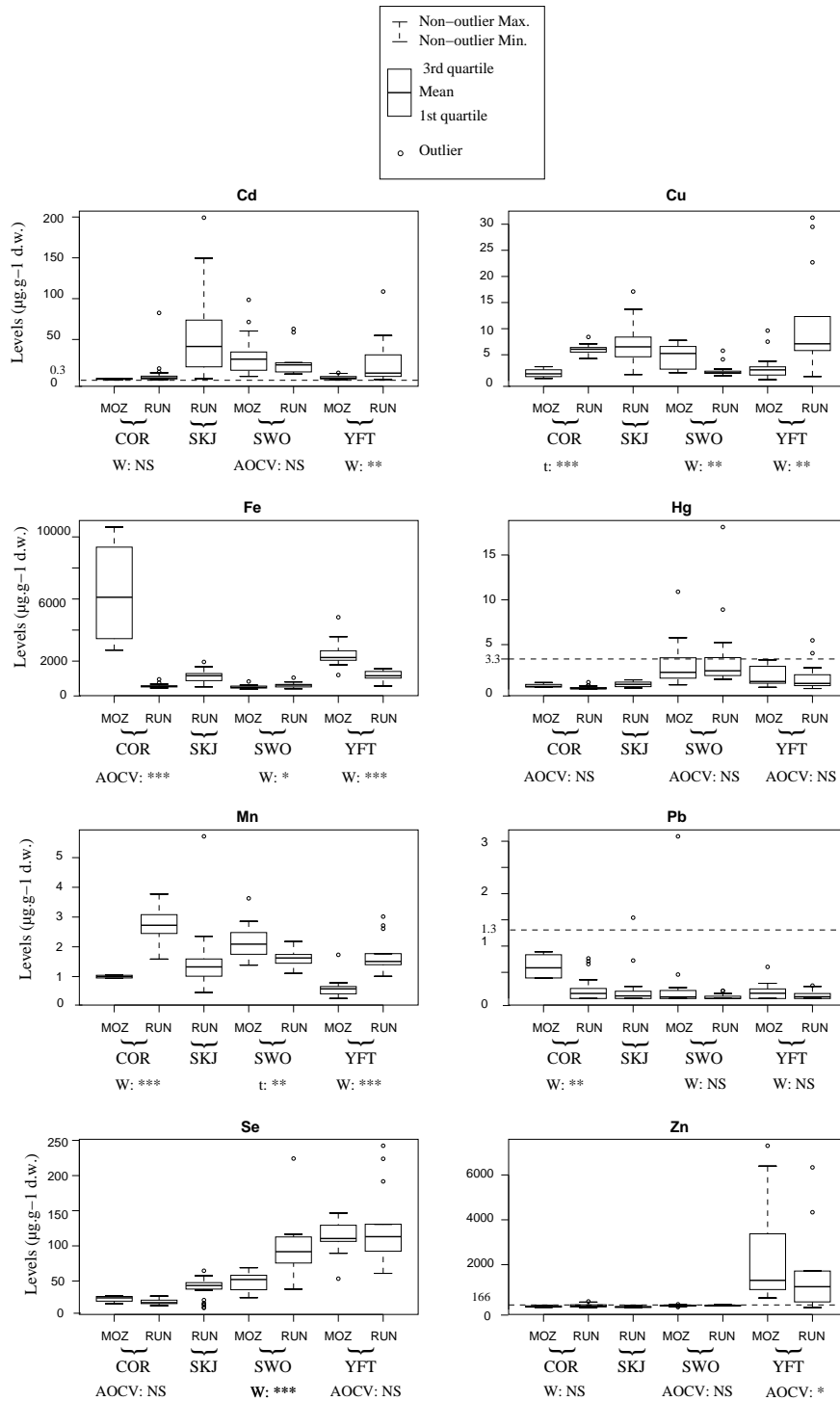
Fig. 4. Comparison of elemental levels ( \mu\text{g}\cdot\text{g}^{-1} d.w.) in kidney of fish caught in the Mozambique Channel (MOZ) and Reunion Island waters (RUN). For each species, the significances of the level differences between both study sites are indicated below the boxplots. Horizontal dotted lines mark the European guidance levels for human consumption. COR: Common Dolphinfinch; SKJ: Skipjack Tunas; SWO: Swordfish; YFT: Yellowfin Tunas; W: Wilcoxon test; t: t-test; AOCV: analysis of covariance; NS: Non significant.
