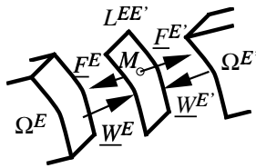
Figure 2. Interface
