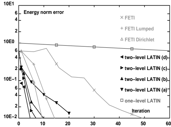
Figure 5: Comparison of methods – error versus iterations
