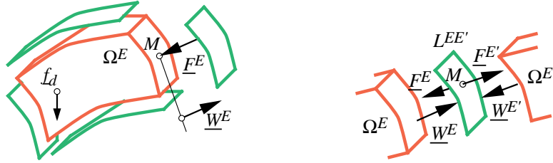
Figure 2. Substructure and interface
