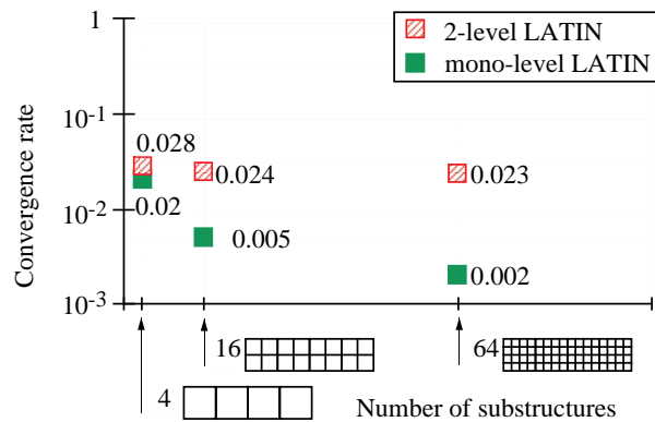
Figure 5. Convergence rate versus number of substructures
