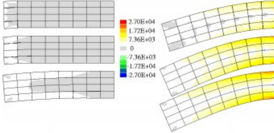
Figure 6: Comparison of solutions at iterations 1,2 and 15 for: a) on the left: the mono-level approach; b) on the right: the micro-macro approach.
