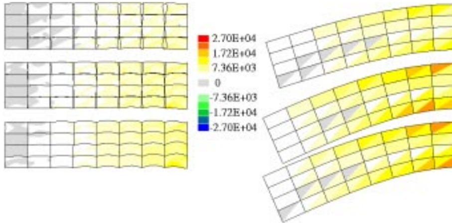
Figure 7: a) on the left: the micro scale solution (with a 10-magnification for displacement); b) on the right: the macro scale solution.
