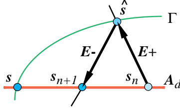
Figure 3. LATIN iterative scheme
