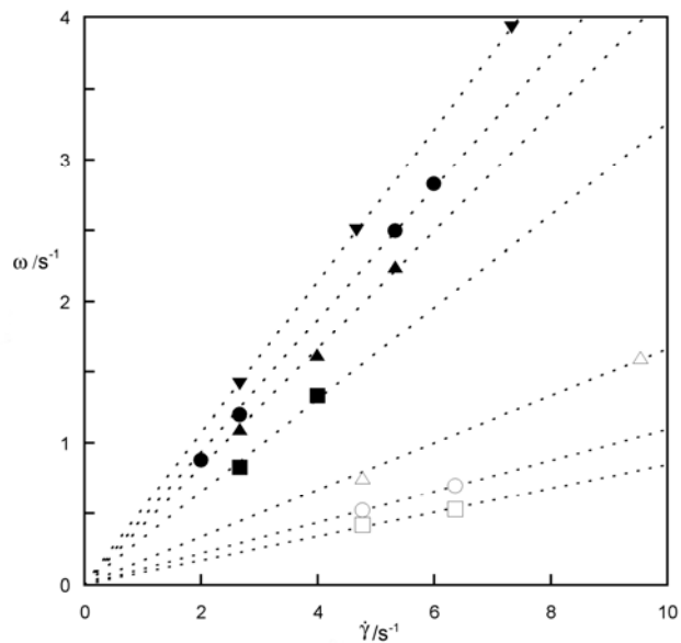
Fig.6 Linear variation of the angular velocity \omega of a circulating marker as a function of the shear rate \dot{\gamma} observed on fixed orbits: \bullet : Ves1; \blacksquare : Ves2; \blacktriangle : Ves3; \blacktriangledown : Ves4; \circ : Ves5; \square : Ves6 and \triangle : Ves7. Dashed lines are linear fit.
