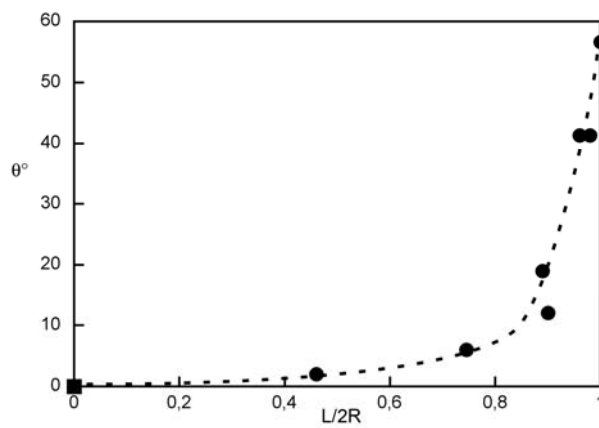
Fig.4 Variation of \theta (defined in Fig. 3) as a function of the aspect ratio L/2R . The dashed line is a guideline for eyes.
