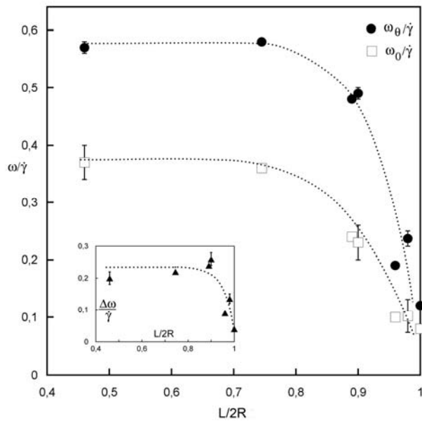
Fig.8 Variation of the reduced angular velocity extrapolated at the stagnation point, \omega_0/\dot{\gamma} , and at the vesicle top, \omega_e/\dot{\gamma} , versus the aspect ratio L/2R . Insert: variation of the reduced gradient angular velocity as a function of L/2R . Dashed lines are guidelines for eyes.
