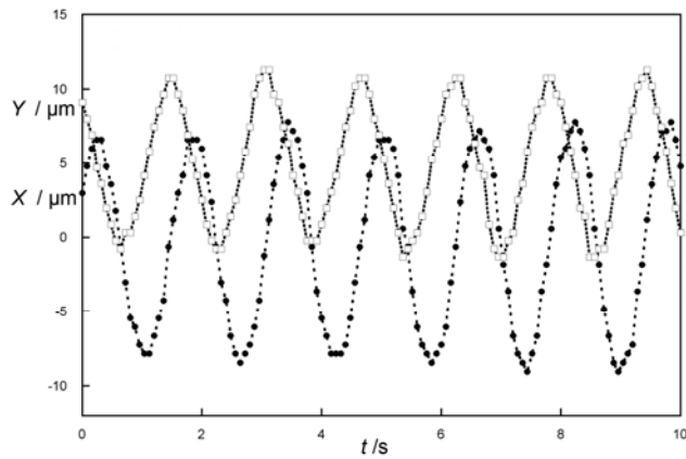
Fig.5 Typical time evolution of the coordinates x (black circles) and y (open squares) of a marker on Ves3 as deduced from side view imaging. The lines are guidelines for eyes.
