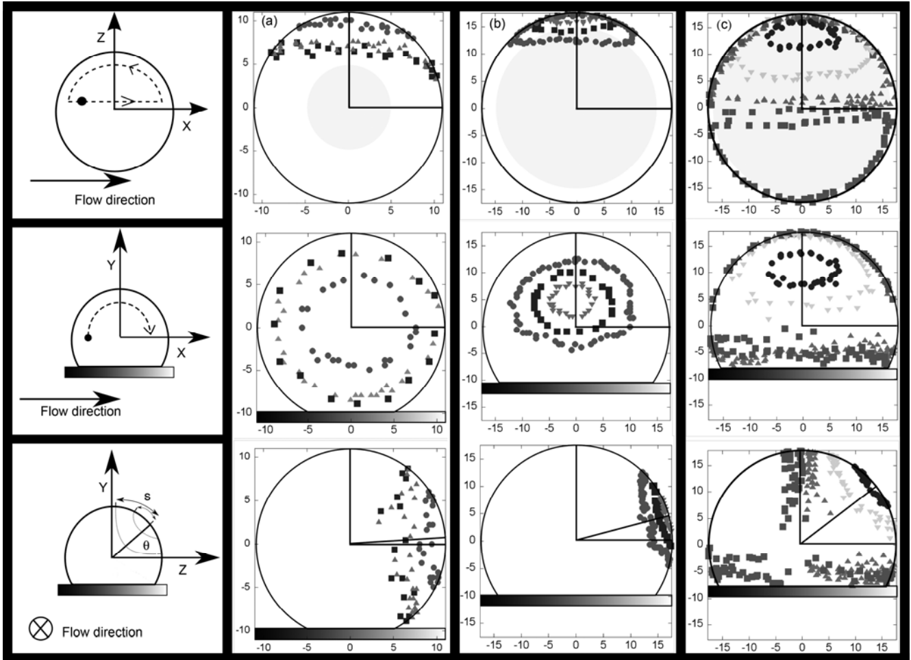
Fig.3 Marker trajectories and streamlines reconstruction for three vesicles. Projection in the plane (x,y) of marker trajectories observed from side view imaging and reconstruction of the corresponding streamlines in (z,y) and (x,z) planes : (a) : Ves1; (b) : Ves3. Projection in the plane (x,z) of marker trajectories observed from bottom view imaging and reconstruction of the corresponding streamlines in (z,y) and (x,y) planes : (c) : Ves5. The grey disc in the (x,z) view represents the contact zone.
