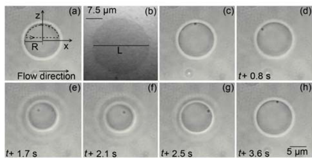
Fig.2 : (a) : Bottom view of Ves5, subjected to a linear shear flow. The dotted line represents the projection of the marker trajectory. (b) : RICM view of ves5 (the scale is different from (a), (c)-(h)). The adhesive zone corresponds to the large homogenous dark disc. (c), (d) and (h): the marker (black dot) avoids the contact zone when approaching the substrate. From (e) to (g) the marker circulates at the vesicle top (the focus varies).
