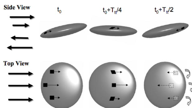
Figure 4: local strain of elastic RBC membrane elements during the rotation of the membrane when the RBC tanktreads
