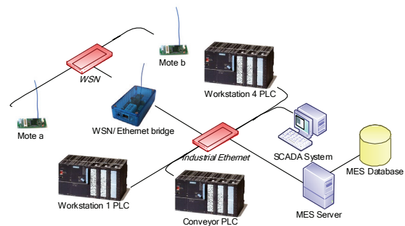
Fig. 8. Principle of the platform technical architecture
