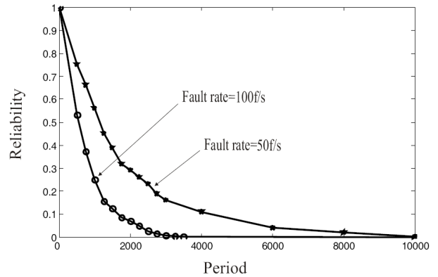
Figure. 5 case 2 reliability
