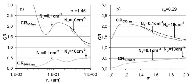
Fig. 2. Colour ratios at 355 ( CR_{355\text{nm}} ) and 1064 nm ( CR_{1064\text{nm}} ) versus r_m (a) and \sigma (b). Reference values for the non varying parameters are, \sigma = 1.45 (a), r_m = 0.29 \mu\text{m} (b), N_o = 0.1 and 10 \text{ cm}^{-3} in both (a) and (b).
