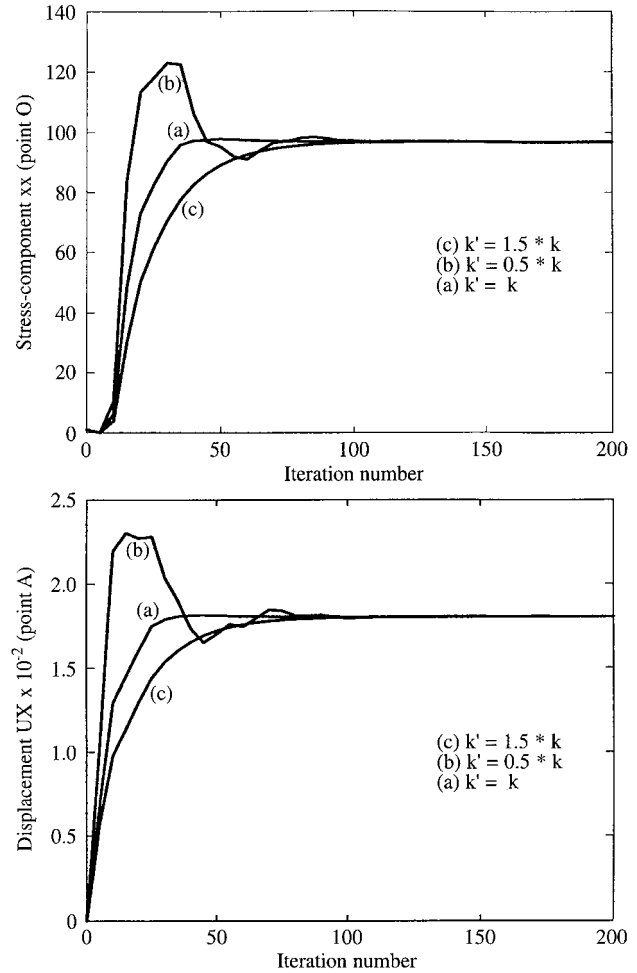
Fig. 7. Evolution of the stress \sigma_{xx} (MPa) and evolution of the displacement U_x (mm) with respect to the iteration number
