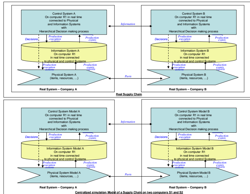
Figure 1.16. Distributed simulation models of a Supply Chain
