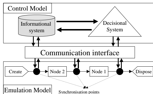
Figure 1.17. Product Driven System Simulation
