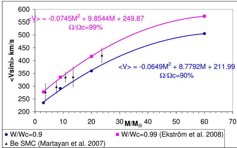
Figure 1. Comparison of average V_{\text{ sini}} distribution for observed Be/Oe stars in the SMC (black points from Martayan et al. 2007) with the theoretical tracks for stars, which display the Be-phenomenon at the SMC metallicity (pink and blue curves are from Ekström et al. 2008).
