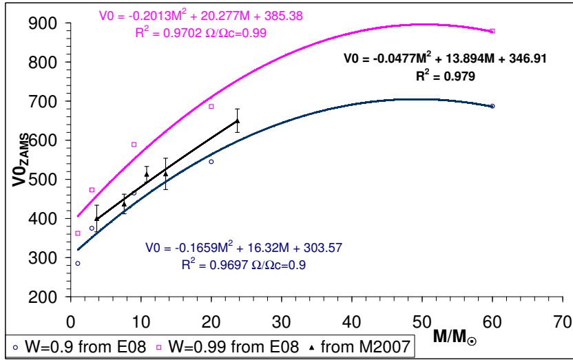
Figure 2. ZAMS rotational velocities distributions for observed Be/Oe stars in the SMC (black points and curve) compared with theoretical distributions from Ekström's et al. (2008).
