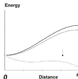
Figure 2: Effect of force on the energy landscape. The figure shows i) bold line : a simple energy well with a barrier (abscissa a ). ii) thin line : the alteration induced by an external force equal to 10 % of the maximal slope of the native curve. The barrier position is not markedly changed, and Kramers's theory may be used, leading to Bell's law. iii) broken line : the alteration induced by an external force equal to about 90% of the maximal slope of the native curve. The barrier is very low and approximations used to derive Bell's law are no longer valid.
