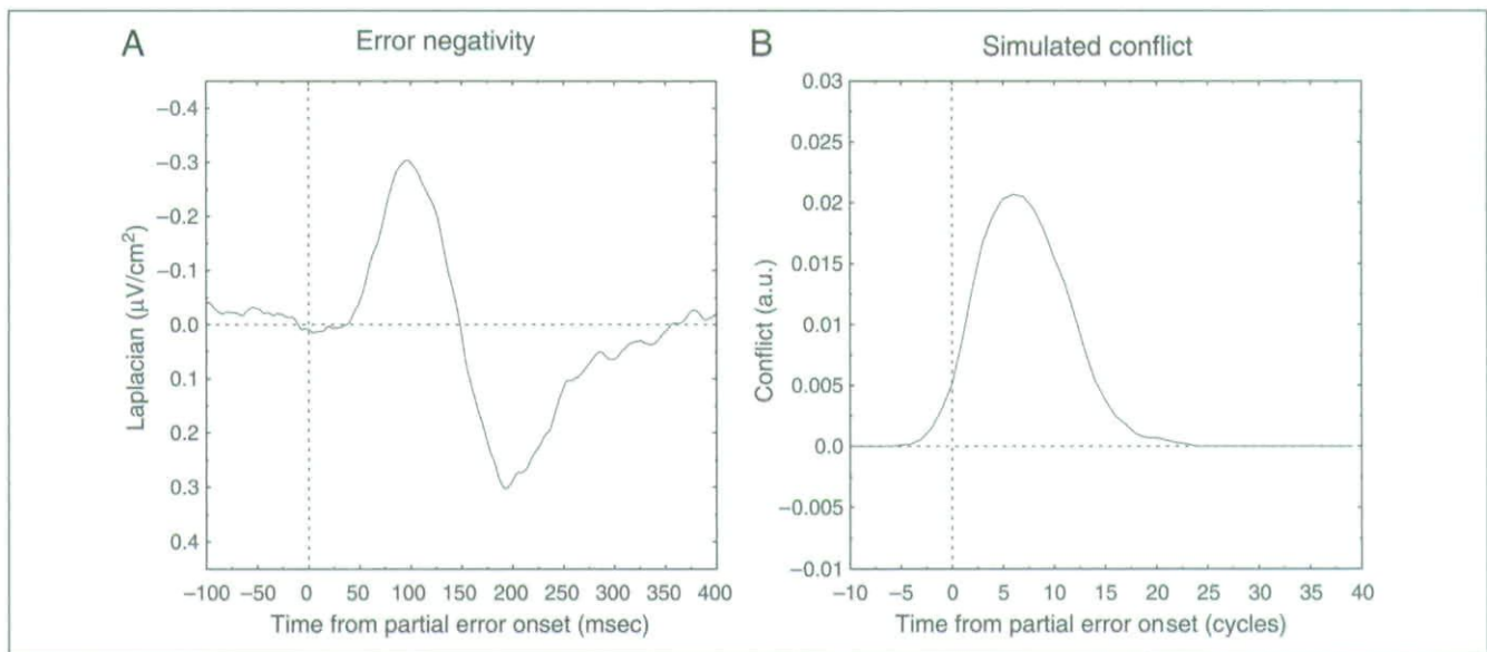
Figure 2. Comparison between grand-averaged N_e and conflict. (A) Amplitude of the Laplacian transformed N_e induced by partial errors as a function of time. The time-zero corresponds to the partial error onset. A clear N_e can be observed starting about 30 msec after incorrect EMG onset and peaking about 100 msec after it. Furthermore, its topography is well localized fronto-centrally (see Figure 8 for the topography of this wave). (B) Grand-averaged conflict as a function of time. Time-zero corresponds to crossing of the partial error threshold. The conflict is clearly maximal just after the partial error, and its timing nicely fits that of the N_e . This confirms that the N_e on partial errors is a valid measure for testing the conflict model predictions.
