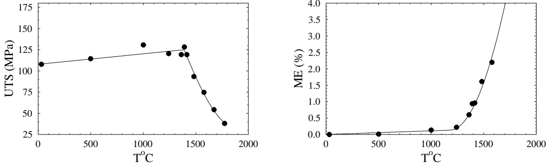
Fig. 2. Ultimate tensile stress (UTS) and maximal elongation (ME) versus temperature for non irradiated UO_2 with 3 % of initial porosity and 8 \mu m grain size (after Canon et al. 1971).
