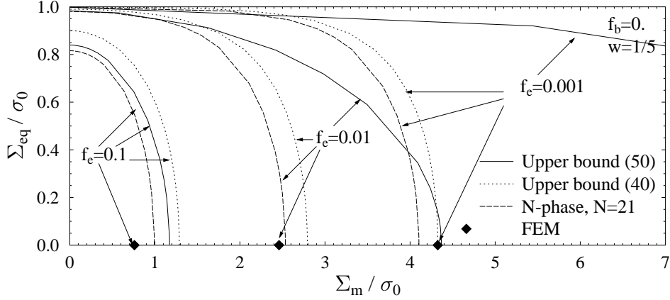
Fig. 14. : Randomly oriented ellipsoidal voids ( w = 1/5 ) in a von Mises matrix ( f_b = 0 ). Drained case ( p_b = p_e = 0 ). Comparison between different predictions: upper bound (40) (dotted line), upper bound (50) (solid line), N-phase estimate ( N = 21 , dashed line), FEM simulations (diamond).
