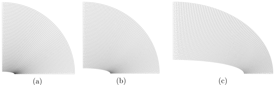
Fig. 13. Meshes used in the unit-cell calculations (a) f_e = 0.001 , w = 1/5 , (b) f_e = 0.01 , w = 1/5 , (c) f_e = 0.1 , w = 1/5 .
