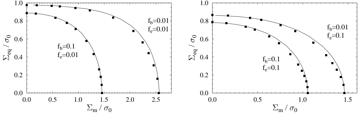
Fig. 9. : Spherical voids in a Gurson matrix. Finite elements simulations (black squares) and N -phase estimate ( N = 21 , solid line), q_3 = q_1 = 1 . Drained case ( p_b = p_e = 0 ).
