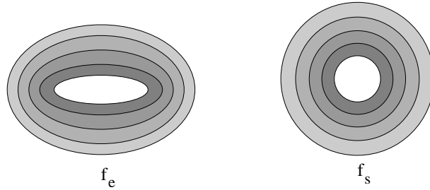
Fig. 10. “ Equivalent porosities ”: the effective elastic properties of the actual configuration (left, porosity f_e ) are identical to the effective properties of the virtual configuration with spherical voids (right, porosity f_s ).
