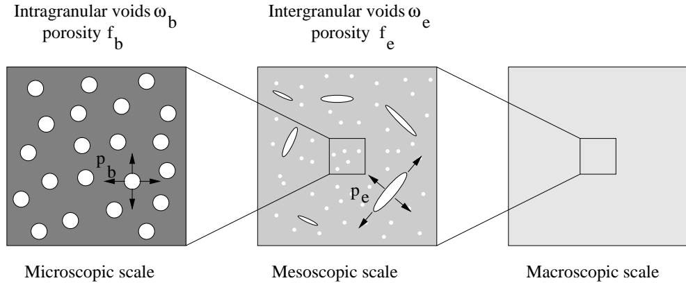
Fig. 3. Up-scaling (or homogenization) procedure.
