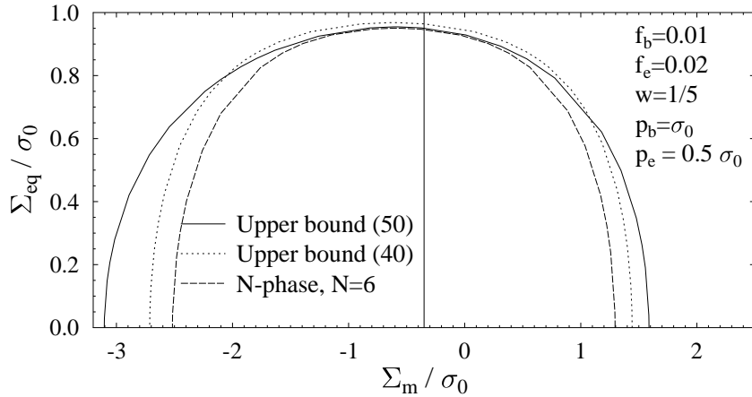
Fig. 12. Gurson matrix containing randomly oriented ellipsoidal voids. f_e = 0.02 , f_b = 0.01 , q_3 = q_1 = 1 , w = 1/5 . Saturated case p_b = \sigma_0 , p_e = \frac{1}{2}\sigma_0 . Comparison between different predictions: upper bound (40) (dotted line), upper bound (50) (solid line), N-phase estimate ( N = 6 , dashed line).
