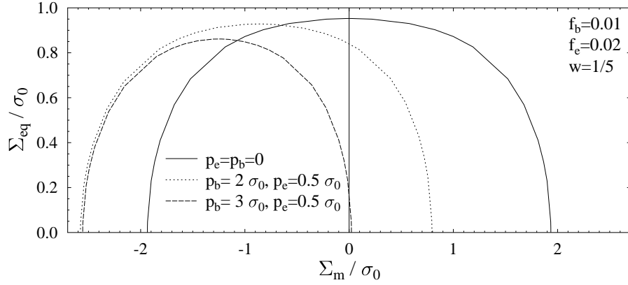
Fig. 16. Gurson matrix containing randomly oriented ellipsoidal voids f_e = 0.02 , f_b = 0.01 , q_3 = q_1 = 1 , w = 1/5 . N -phase estimate of the effective flow surface ( N = 6 ). Comparison between the drained case ( p_b = p_e = 0 , solid line) and two saturated cases p_b = 2\sigma_0 , p_e = \frac{1}{2}\sigma_0 (dotted line) and p_b = 3\sigma_0 , p_e = \frac{1}{2}\sigma_0 (dashed line).
