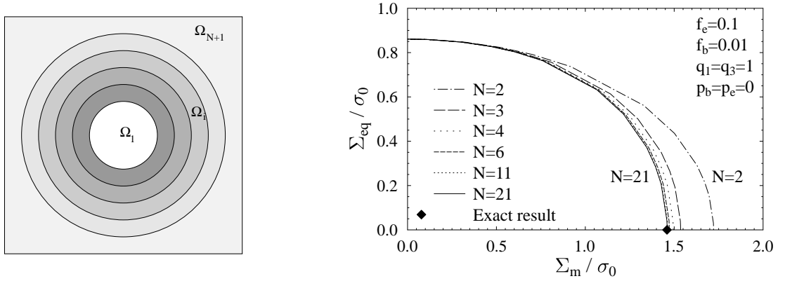
Fig. 6. Left: multi-layered inclusion in an infinite matrix. Right: influence of the number of subdomains on the accuracy of the N -phase model. f_e = 0.1 , f_b = 0.01 , q_3 = q_1 = 1 . Drained case ( p_b = p_e = 0 ). Diamond: exact result (D.7).
