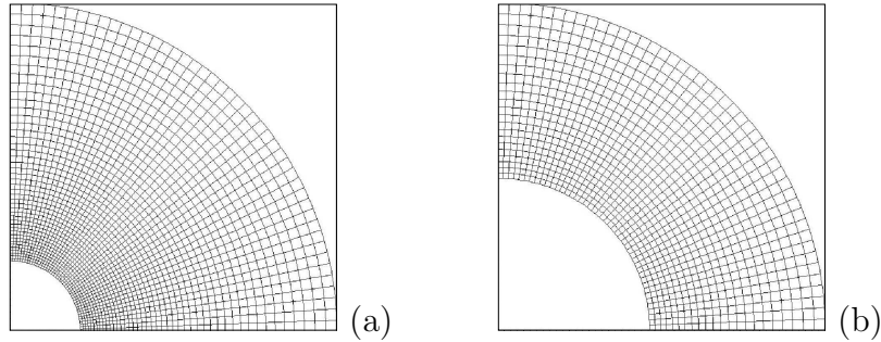
Fig. 8. Finite element meshes used in the unit-cell calculations: (a) f_e = 0.01 , (b) f_e = 0.1 .
