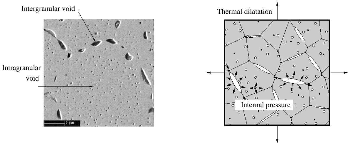
Fig. 1. Left: micrography of irradiated \text{UO}_2 ( 33\ \text{GW j/T} ) after heat treatment at 2000^0\ \text{K} during 3 hours (Dubourg et al., 2005). Right: swelling of \text{UO}_2 during an accident. Development of thermal strains and internal pressures inside the cavities.
