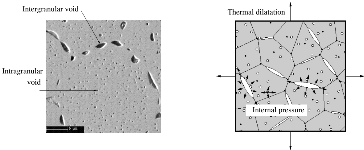
Fig. 1. Left: micrograph of irradiated \text{UO}_2 (33 GW j/T) after heat treatment at 2000^0\text{K} during 3 hours (Dubourg et al., 2005). Right: swelling of \text{UO}_2 during an accident. Development of thermal strains and internal pressures inside the cavities.
