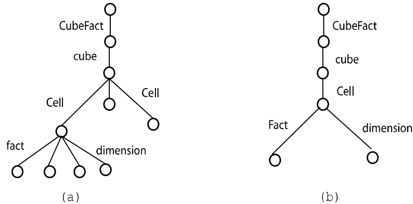
Figure 3: Facts.xml structure (a) and corresponding 1-index (b)
