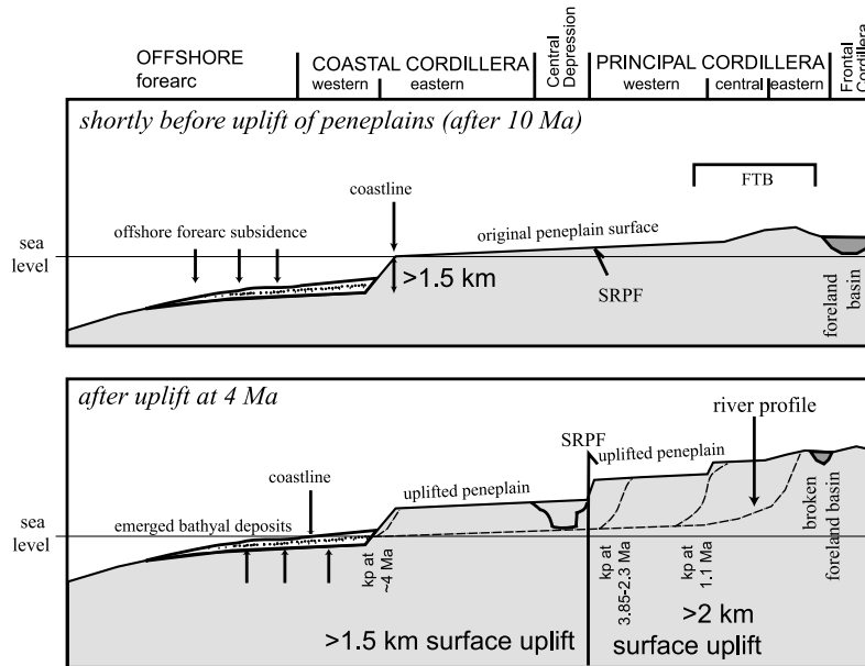
(a) Model 1: uplift at ~4 Ma (coupled Coastal Cordillera)
