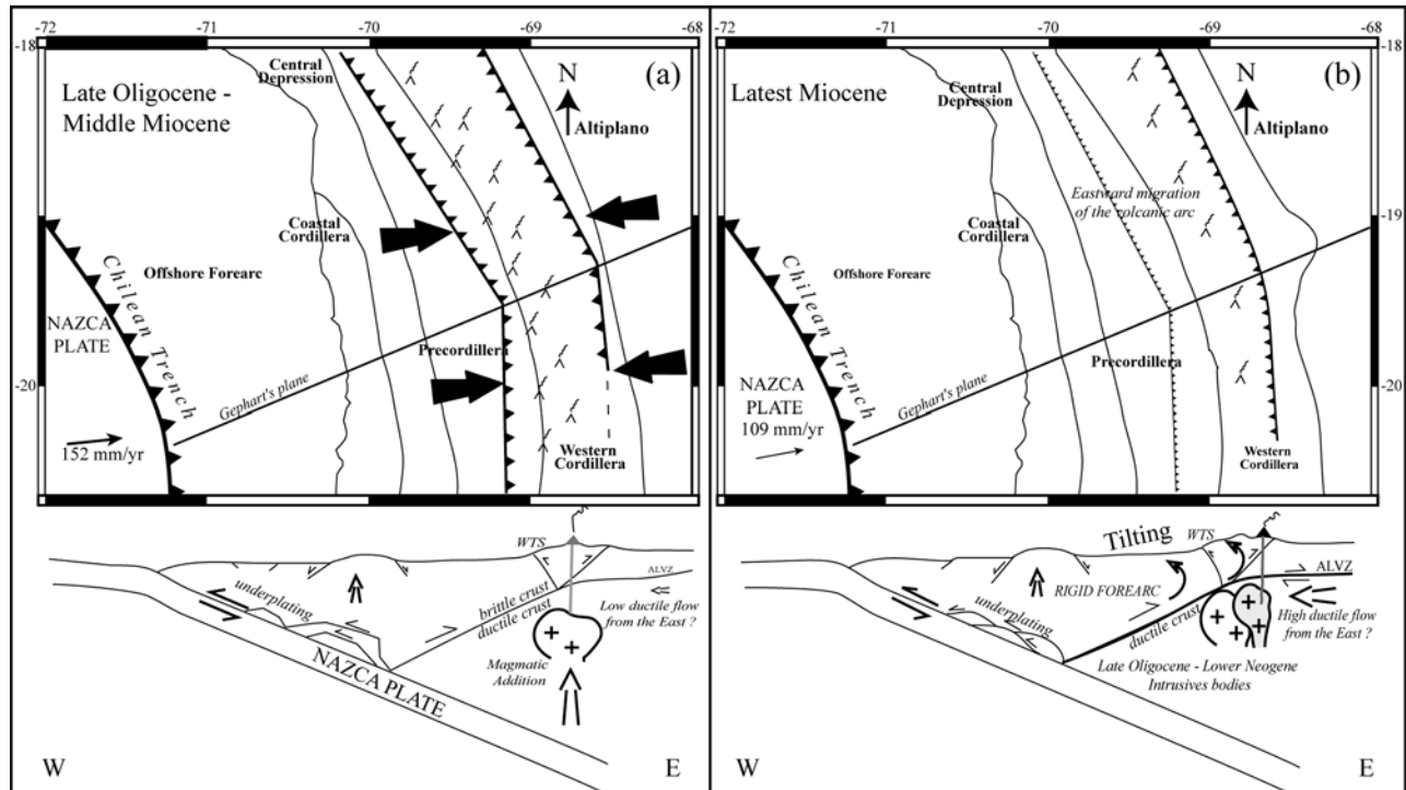
Figure 18. Schematic evolution of the uplift of the western side of the Altiplano in northern Chile. (a) Tectonic situation between 26 and 8 Ma, where rapid and orthogonal plate convergence was the main tectonic feature. During this time, large volumes of magma were emplaced below the Precordillera and Western Cordillera. Little ductile flow of the lower crust is expected for this time. (b) Tectonic situation in the latest Miocene. At this time, nearly 1–3 km of surface uplift occurred within the Altiplano as a result of crustal thickening, probably triggered by the hypothetical ductile flow of the lower crust coming from the sub-Andean zone to the Altiplano. This uplift is marked by westward forearc tilting. Morphologic units (trench, coastline, Coastal Cordillera, Central Depression, Precordillera, and Western Cordillera) are reported in their present-day location. Plate convergence vector is after Somoza [1998].
