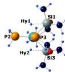
Figure 3. View of the transition state corresponding to the inversion of the Si-H bonding modes
