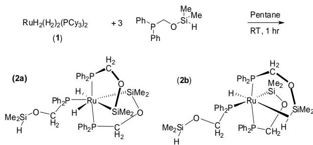
Scheme 1. Synthesis of 2 represented by two arrested structures ( 2a,b ).
