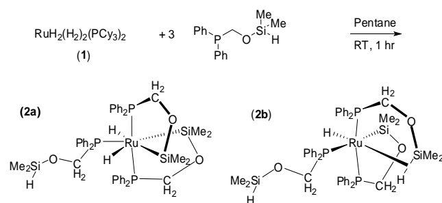
Scheme 1. Synthesis of 2 represented by two arrested structures ( 2a,b ).
