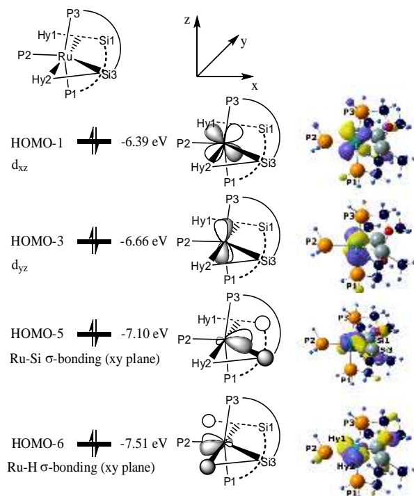
Figure 2. Selected occupied orbitals of model complex
