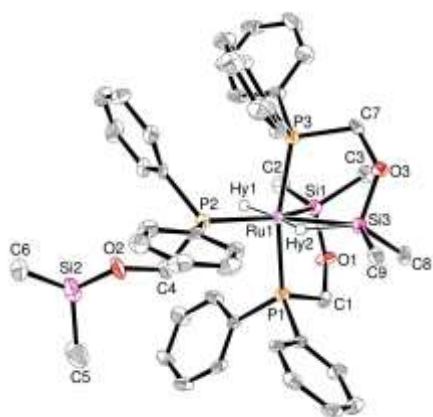
Figure 1. Molecular structure of \text{Ru}(\text{PPh}_2\text{CH}_2\text{OSiMe}_2\text{H})_3 ( 2 ). Thermal ellipsoid plot (50% probability surface). Hydrogen atoms except hydrides have been omitted for clarity.
