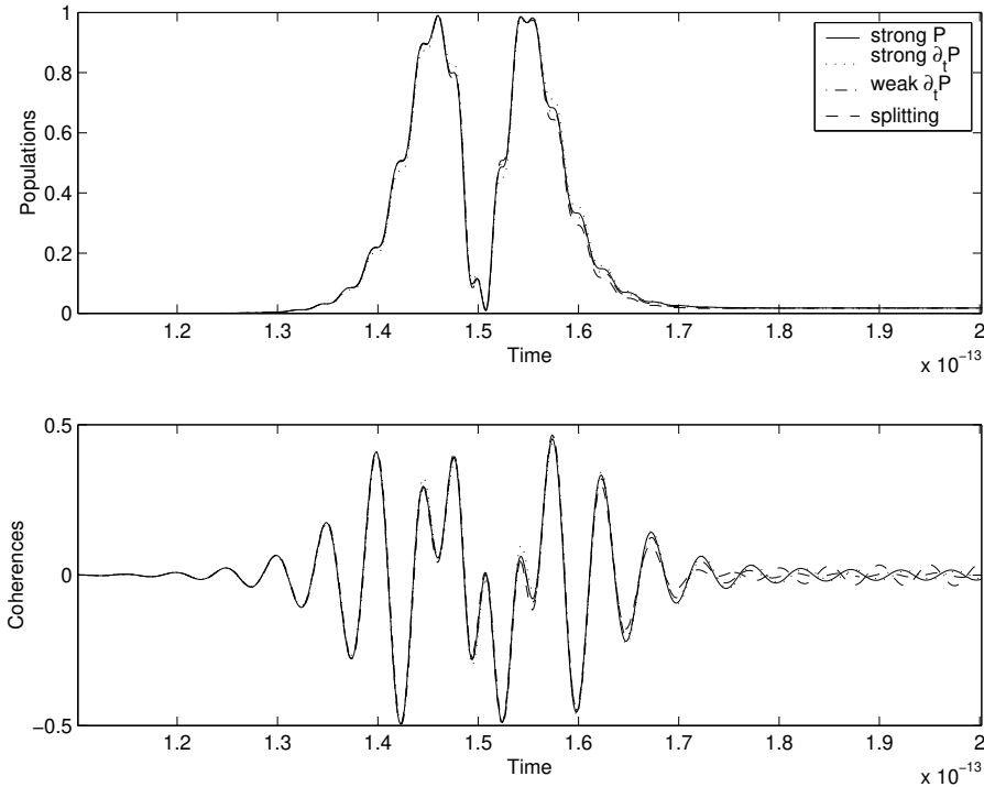
Figure 1: SIT : comparison of the different schemes on a 20 points per wavelength grid. Time evolution of \rho_{11} and |\rho_{12}| .
