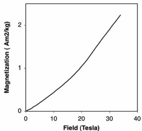
Figure 3. Induced magnetization measured at 4.2 K in the LNCMP pulse system on GT unoriented massive sample. Spin-flop transition corresponds to the slope change around 20 T; see Coey et al. [1995] for details on such curves.
