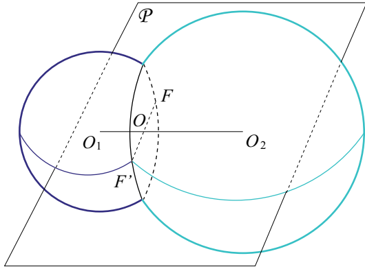
Figure 6. Intersecting two spheres.
