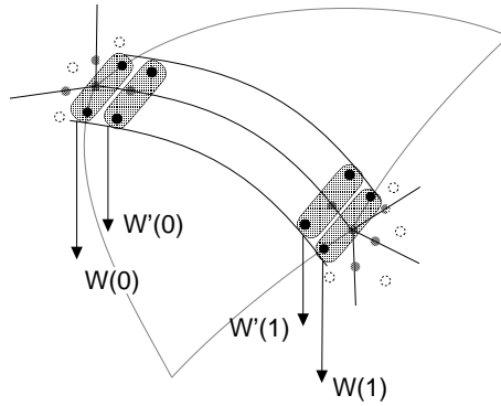
Figure 8: G^1 compatible tangent ribbons at end points.
