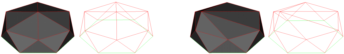
Figure 15: left: regular mesh, right: deformed mesh.
