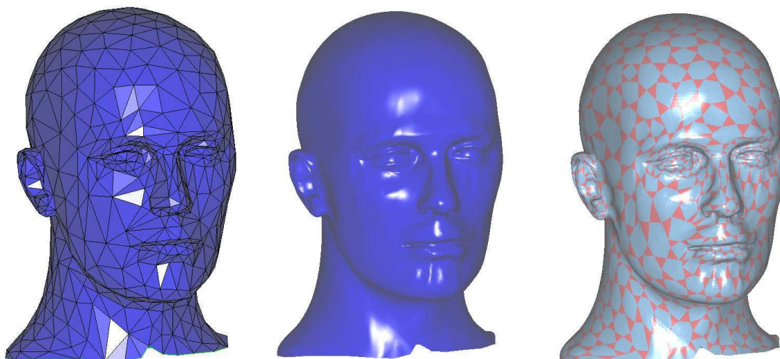
Figure 1: Mannequin, mesh left, G^1 surface middle, control-polygons right.
