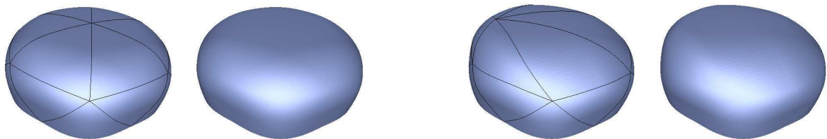
Figure 17: interpolation with arbitrary choice of tangents.
