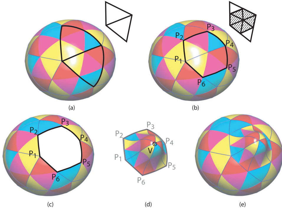
Fig. 7. Local Surface Refinement
