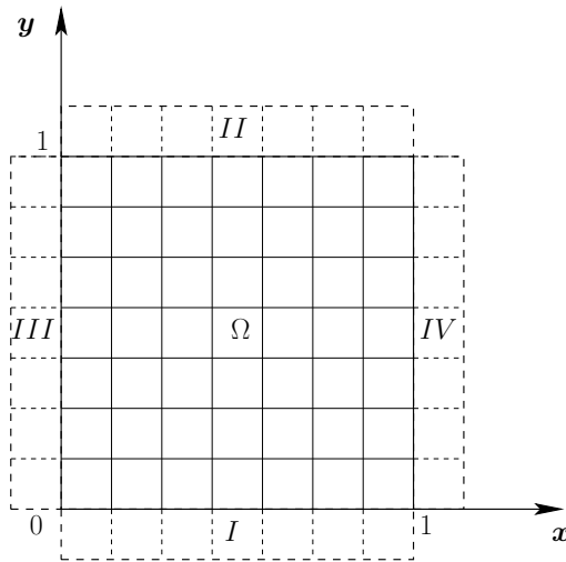
Figure 2: Schematics of the computational domain.
