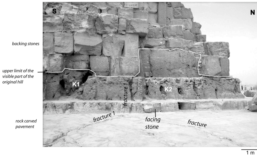
Figure 15. Kheops Pyramid. View of the NE corner located on figure 11. The white line outlines the visible part of the natural rock affected by fractures and solution phenomena. K1: karst natural fracture, K2: cavities showing advanced dissolution processes along the stratum surface.
