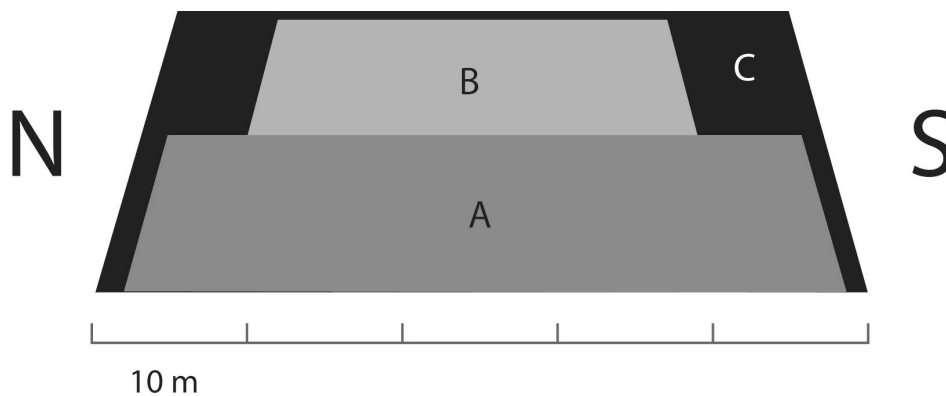
Figure 7. Reconstitution of the initial volume of queen Kentkawes mastaba (C), including the present geometry of the original hill (A) and the reconstituted constructed part (B).
