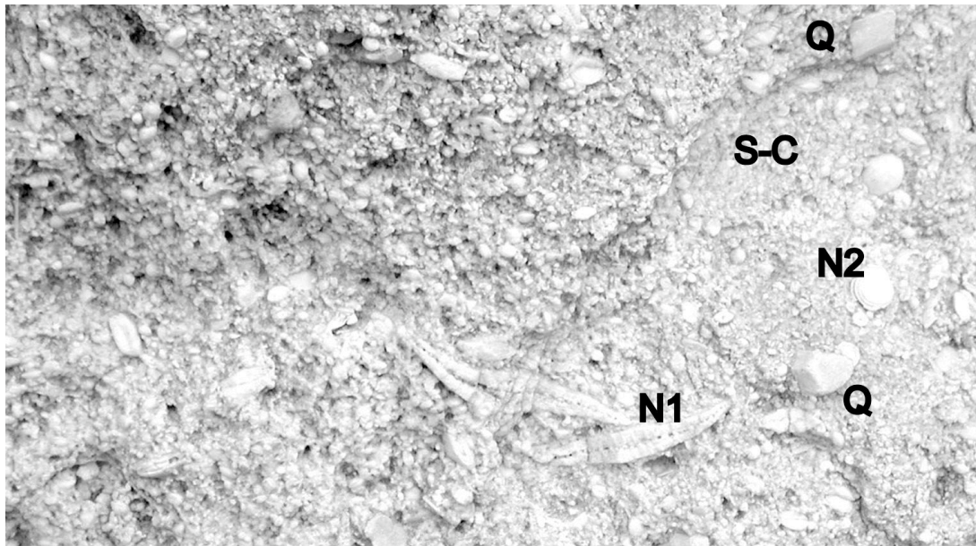
Figure 13. Khephren Pyramid. Microfacies of the wackestone levels of the substratum, including the two sets of Nummulites Gizehensis . Q: quartz gravel, N: nummulites, S-C: sand and clay.
