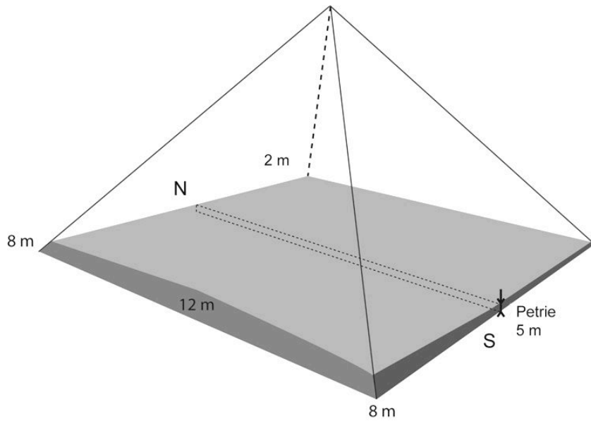
Figure 18. Khephren Pyramid. Three-dimensional representation of the visible part of the original hill, including Petrie's observations.
