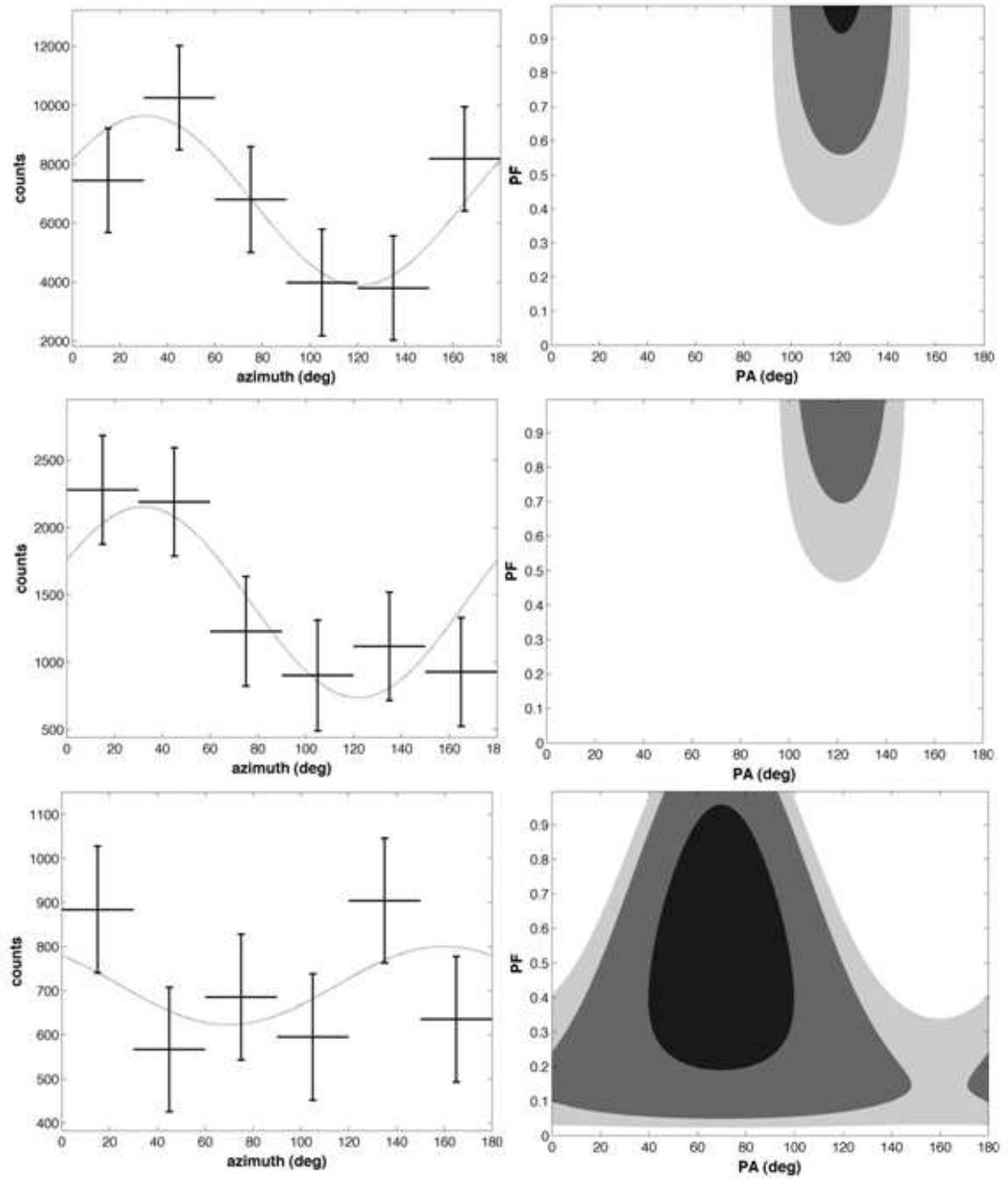
Fig. 2.— Azimuthal profile, modulation angle, PA, and fraction, PF = a_0/a_{100} , measured for the Crab data between 200 and 800 keV, in the off-pulse (top), off-pulse and bridge (middle), and two-peak (bottom) phase intervals. The error bars for the profile are at one sigma. The 68%, 95%, and 99% confidence regions are shaded from dark to light gray.
