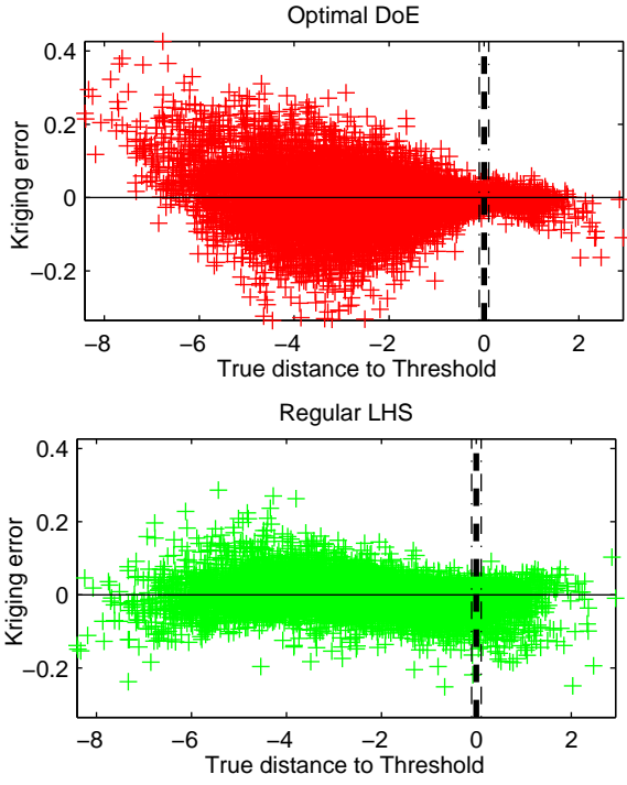
Fig. 5. Comparison of error distribution for two 90-point DoEs: optimal DoE (top) and classical LHS (bottom). The x-axis is the difference between the true function and the threshold, the y-axis is the error. Three vertical bars are drawn at -2\sigma_\varepsilon , 0 and +2\sigma_\varepsilon for the target region. The error is on average smaller for the LHS design, but the optimal DoE reduces substantially the error in the target region.
