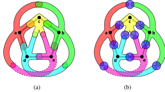
Figure 3: (a) the complete graph K_5 generates an example of a diagram that is not Eulerian, as any attempt to draw it generates disconnected zones. In fact, we will have to disconnect the zones d and e (see fig. 4.a) to draw the dashed link. The same graph is drawable, if we allow duplicated zones. (b) an example of a graph that is not drawable whitout disconnecting classes, even if allowing disconnected zones. The circular sets are all meant to be distinct. This time any attempt to draw the dashed link brings undesired overlaps, so the class E will have to remain disconnected.
