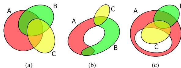
Figure 1: Euler diagrams as studied by different authors. (a) shows Euler diagrams as studied in [5]. They do not permit overlapping lines and multiple-line crossing points. (b) shows the more general Euler diagrams studied in [3]. Multiple line crossing point and overlapping boundary are allowed, as well as disconnected overlaps between the same sets. (c) shows Extended Euler diagrams (EED) as defined in [9]. Holes inside the sets are permitted.
