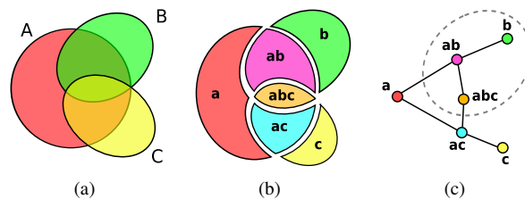
Figure 2: From the Euler diagram to the intersection graph. (a) the original diagram. (b) individuation of the diagram zones. (c) the resulting intersection graph. The dashed line is not part of the graph, but shows how to reverse the procedure. For drawing the boundary of the class B we need to enclose the nodes b, ab, abc and intersect the edges (a, ab), (ac, abc) .
