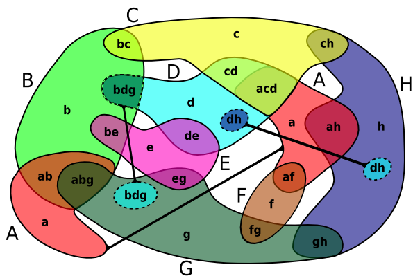
Figure 8: a Euler representation example. The diagram structure is not planar (it has a K_5 minor), so it cannot be represented with Euler diagrams. The Euler representation proposed uses zone duplication for bdg and dh , and has a disconnected class A .
