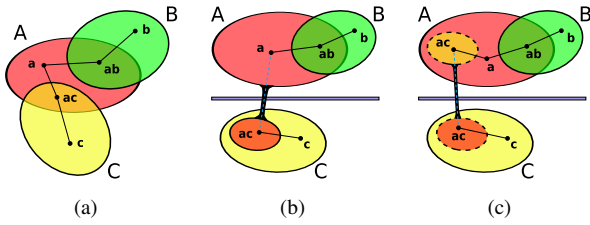
Figure 5: Visualisation of disconnected classes. (a) the original diagram, showing the relationships we aim to represent. Let us suppose the zones ac , c are not directly reachable from the others. (b) shows a possible way to depict a link between separated zones of the same class. This representation does not show straight away that the class A contains ac , especially if they are positioned far apart from each other. (c) shows the duplication of the zone ac and its nodes. A spotted boundary is used to indicate that the zone has been cloned and not simply represented with separated regions. This representation shows in a more immediate way that the classes A and C interact with each other, as well as it shows all the elements of the same class in the same connected area.
