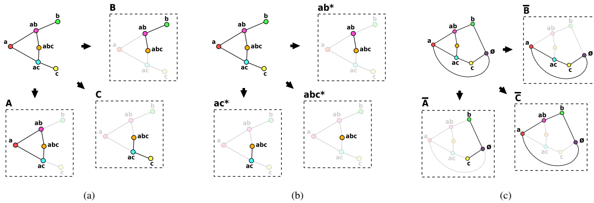
Figure 7: Some tests on the intersection graph. (a) checking that all the class schemas are connected. (b) checking that subgraphs induced by the nodes containing any possible subset of classes are connected. Here the subgraphs induced by the nodes containing ab , ac , and abc are shown. Together with the ones containing a , b , and c (that correspond exactly to the class schemas in the previous picture), they are all the possible non empty subgraphs of this kind. (c) checking that the complementar class schemas are connected. At this point we need to consider also a node associated to the external area, that will always be part of the complementar class schemas.
