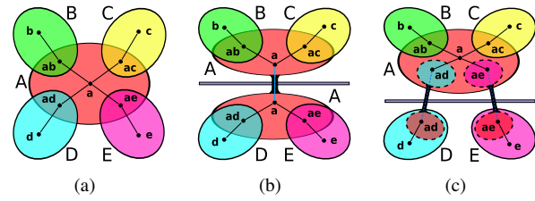
Figure 6: Another example of disconnected classes. (a) the original diagram, built without particular constraints. Let us now assume class D and E are not reachable from A , B , C . (b) the diagram obtained when representing the zone a as two separated regions. In this case, node duplication is generally not meaningful for a better comprehension of the diagram. (c) the same graph obtained duplicating the zones ad and ae and their nodes. Again, node duplication can be made clear by using a dashed line for the boundary. Although this solution allows us to see all the nodes of the same class in a connected region, it tends to be less readable than the previous one because of the greater number of extra links required.
