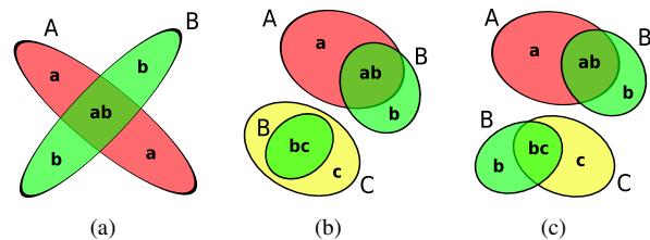
Figure 4: (a) a diagram with disconnected zones, as zone a and zone b are represented by separated regions divided by the zone ab . (b) a diagram with disconnected classes, as class B has the zones ab, b separated from zone bc . (c) a diagram with disconnected zones and classes, as zone b is duplicated and the class B is disconnected.
